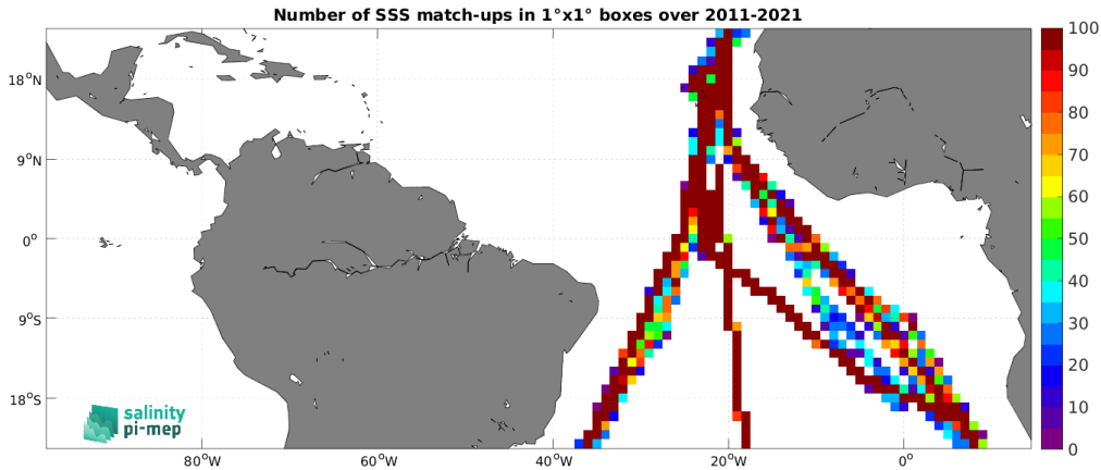
Figure 4: Number of SSS match-ups between TSG (Polarstern) SSS and the SMOS SSS L4 v2 - Daily (BEC) SSS product for the Tropical Atlantic Ocean Pi-MEP region over 1^\circ \times 1^\circ boxes and for the full satellite product period.
