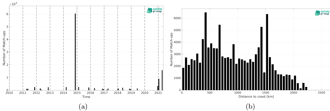
Figure 1: Number of match-ups between TSG (Polarstern) and SMOS SSS L4 v2 - Daily (BEC) SSS as a function of time (a) and as function of the distance to coast (b) over the Tropical Atlantic Ocean Pi-MEP region and for the full satellite product period.
