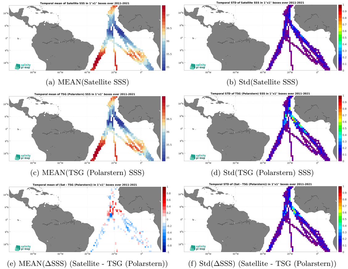
Figure 6: Temporal mean (left) and Std (right) of SSS from SMOS SSS L4 v2 - Daily (BEC) (top), TSG (Polarstern) (middle), and of \Delta\text{SSS} (Satellite - TSG (Polarstern)). Only match-up pairs are used to generate these maps.
