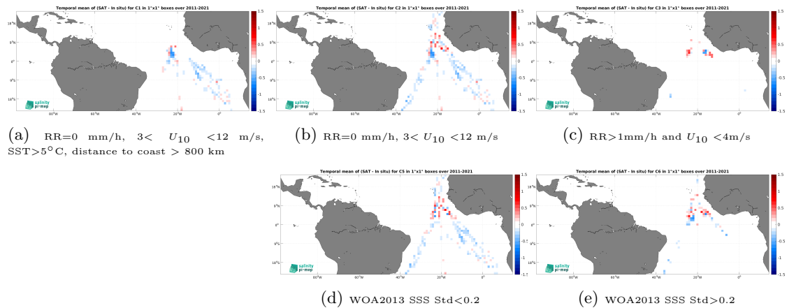
Figure 12: Temporal mean gridded over spatial boxes of size 1^\circ \times 1^\circ of \Delta\text{SSS} (SMOS SSS L4 v2 - Daily (BEC) - TSG (Polarstern)) for 5 different subdatasets corresponding to:RR=0 mm/h, 3 < U_{10} < 12 m/s, SST >5^\circ\text{C} , distance to coast > 800 km (a), RR=0 mm/h, 3 < U_{10} < 12 m/s (b), RR >1 mm/h and U_{10} < 4 m/s (c), WOA2013 SSS Std <0.2 (d), WOA2013 SSS Std >0.2 (e).
