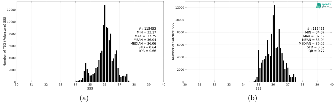
Figure 2: Histograms of SSS from TSG (Polarstern) (a) and SMOS SSS L4 v2 - Daily (BEC) (b) considering all match-up pairs per bins of 0.1 over the Tropical Atlantic Ocean Pi-MEP region and for the full satellite product period.
