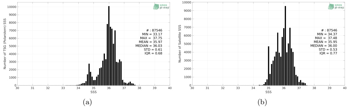
Figure 2: Histograms of SSS from TSG (Polarstern) (a) and SMOS SSS L4 v2 - Daily (BEC) (b) considering all match-up pairs per bins of 0.1 over the Tropical Atlantic Ocean Pi-MEP region and for the full satellite product period.
