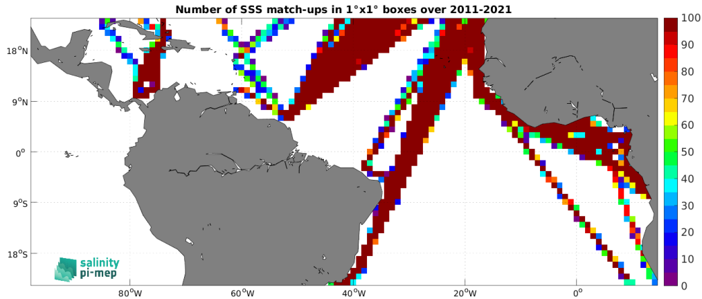
Figure 5: Number of SSS match-ups between TSG (LEGOS-DM) SSS and the SMOS SSS L4 v2 - Daily (BEC) SSS product for the Tropical Atlantic Ocean Pi-MEP region over 1^\circ \times 1^\circ boxes and for the full satellite product period.
