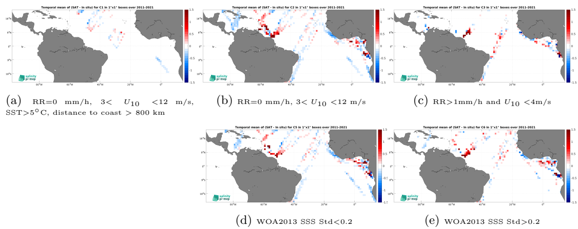
Figure 14: Temporal mean gridded over spatial boxes of size 1^\circ \times 1^\circ of \Delta\text{SSS} (SMOS SSS L4 v2 - Daily (BEC) - TSG (LEGOS-DM)) for 5 different subdatasets corresponding to:RR=0 mm/h, 3 < U_{10} < 12 m/s, SST>5°C, distance to coast > 800 km (a), RR=0 mm/h, 3 < U_{10} < 12 m/s (b), RR>1mm/h and U_{10} < 4 m/s (c), WOA2013 SSS Std<0.2 (d), WOA2013 SSS Std>0.2 (e).
