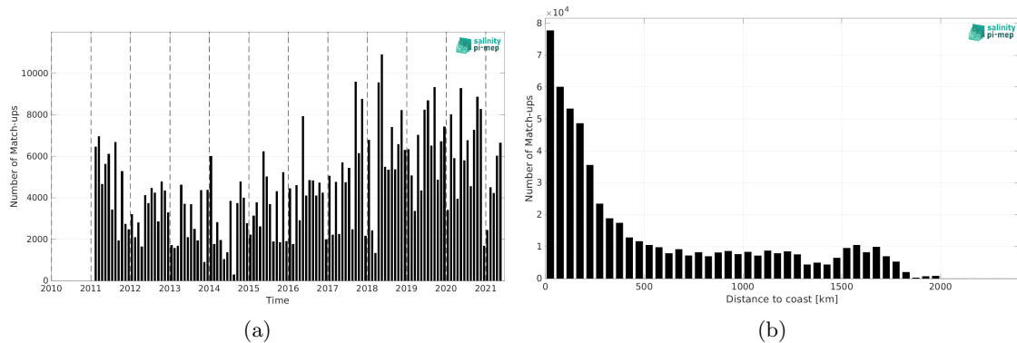
Figure 2: Number of match-ups between TSG (LEGOS-DM) and SMOS SSS L4 v2 - Daily (BEC) SSS as a function of time (a) and as function of the distance to coast (b) over the Tropical Atlantic Ocean Pi-MEP region and for the full satellite product period.
