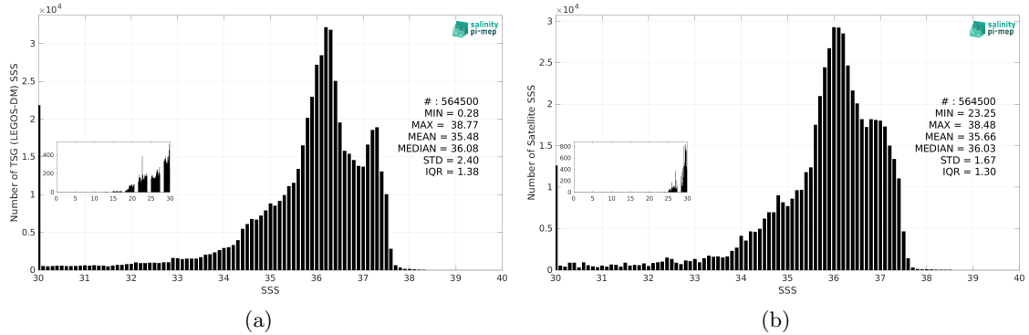
Figure 3: Histograms of SSS from TSG (LEGOS-DM) (a) and SMOS SSS L4 v2 - Daily (BEC) (b) considering all match-up pairs per bins of 0.1 over the Tropical Atlantic Ocean Pi-MEP region and for the full satellite product period.
