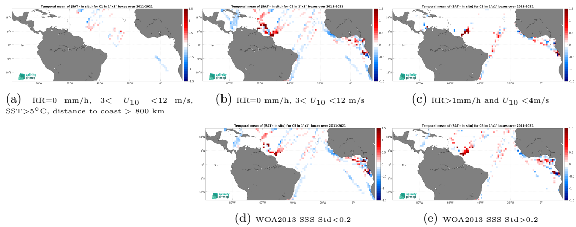
Figure 14: Temporal mean gridded over spatial boxes of size 1^\circ \times 1^\circ of \Delta\text{SSS} (SMOS SSS L4 v2 - Daily (BEC) - TSG (LEGOS-DM)) for 5 different subdatasets corresponding to:RR=0 mm/h, 3 < U_{10} < 12 m/s, SST>5°C, distance to coast > 800 km (a), RR=0 mm/h, 3 < U_{10} < 12 m/s (b), RR>1mm/h and U_{10} < 4 m/s (c), WOA2013 SSS Std<0.2 (d), WOA2013 SSS Std>0.2 (e).
