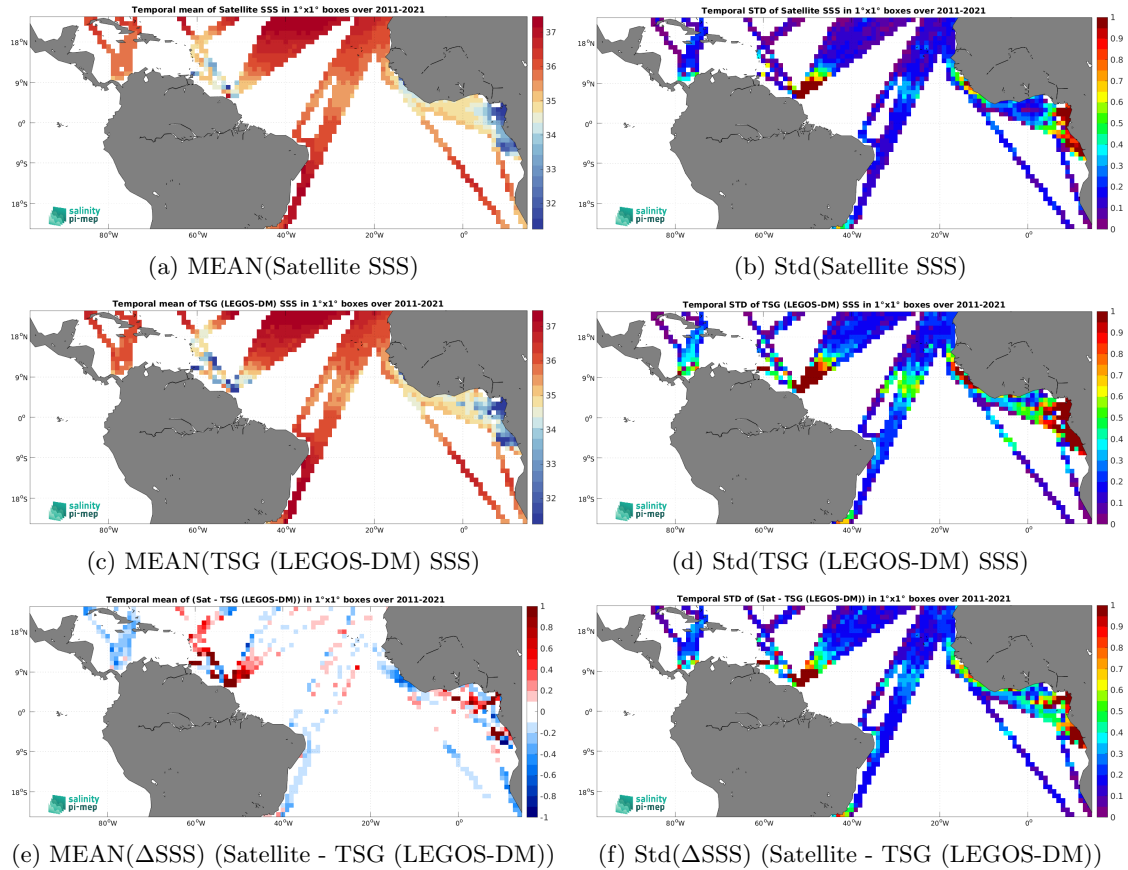
Figure 7: Temporal mean (left) and Std (right) of SSS from SMOS SSS L4 v2 - Daily (BEC) (top), TSG (LEGOS-DM) (middle), and of \Delta\text{SSS} (Satellite - TSG (LEGOS-DM)). Only match-up pairs are used to generate these maps.
