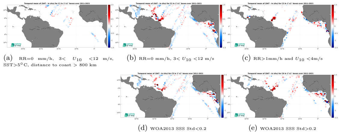
Figure 12: Temporal mean gridded over spatial boxes of size 1^\circ \times 1^\circ of \Delta\text{SSS} (SMOS SSS L4 v2 - Daily (BEC) - TSG (LEGOS-DM)) for 5 different subdatasets corresponding to:RR=0 mm/h, 3 < U_{10} < 12 m/s, SST >5^\circ\text{C} , distance to coast > 800 km (a), RR=0 mm/h, 3 < U_{10} < 12 m/s (b), RR >1 mm/h and U_{10} < 4 m/s (c), WOA2013 SSS Std <0.2 (d), WOA2013 SSS Std >0.2 (e).
