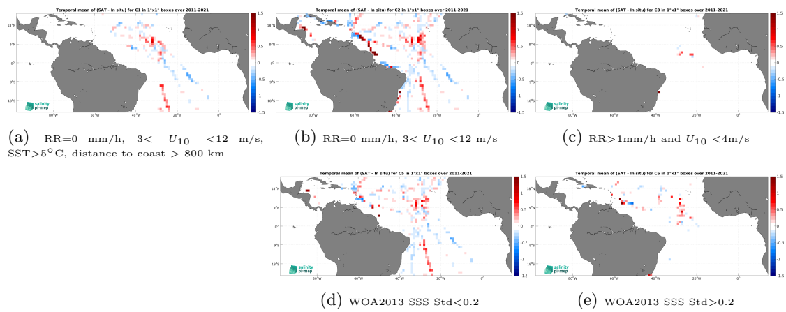
Figure 14: Temporal mean gridded over spatial boxes of size 1^\circ \times 1^\circ of \Delta\text{SSS} (SMOS SSS L4 v2 - Daily (BEC) - TSG (GOSUD-Sailing-ship)) for 5 different subdatasets corresponding to:RR=0 mm/h, 3 < U_{10} < 12 m/s, SST >5^\circ\text{C} , distance to coast > 800 km (a), RR=0 mm/h, 3 < U_{10} < 12 m/s (b), RR >1 mm/h and U_{10} < 4 m/s (c), WOA2013 SSS Std <0.2 (d), WOA2013 SSS Std >0.2 (e).
