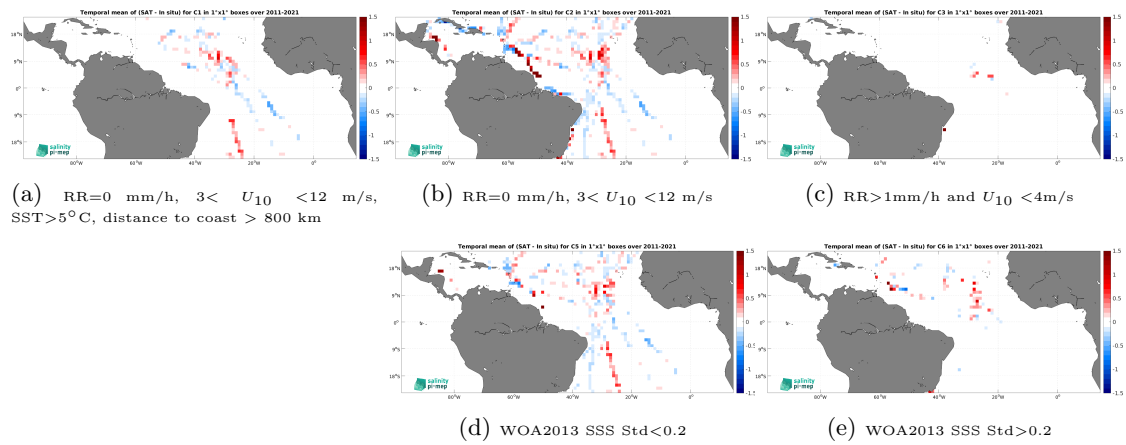
Figure 14: Temporal mean gridded over spatial boxes of size 1^\circ \times 1^\circ of \Delta\text{SSS} (SMOS SSS L4 v2 - Daily (BEC) - TSG (GOSUD-Sailing-ship)) for 5 different subdatasets corresponding to:RR=0 mm/h, 3 < U_{10} < 12 m/s, SST >5^\circ\text{C} , distance to coast > 800 km (a), RR=0 mm/h, 3 < U_{10} < 12 m/s (b), RR >1 mm/h and U_{10} < 4 m/s (c), WOA2013 SSS Std <0.2 (d), WOA2013 SSS Std >0.2 (e).
