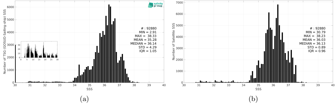
Figure 3: Histograms of SSS from TSG (GOSUD-Sailing-ship) (a) and SMOS SSS L4 v2 - Daily (BEC) (b) considering all match-up pairs per bins of 0.1 over the Tropical Atlantic Ocean Pi-MEP region and for the full satellite product period.
