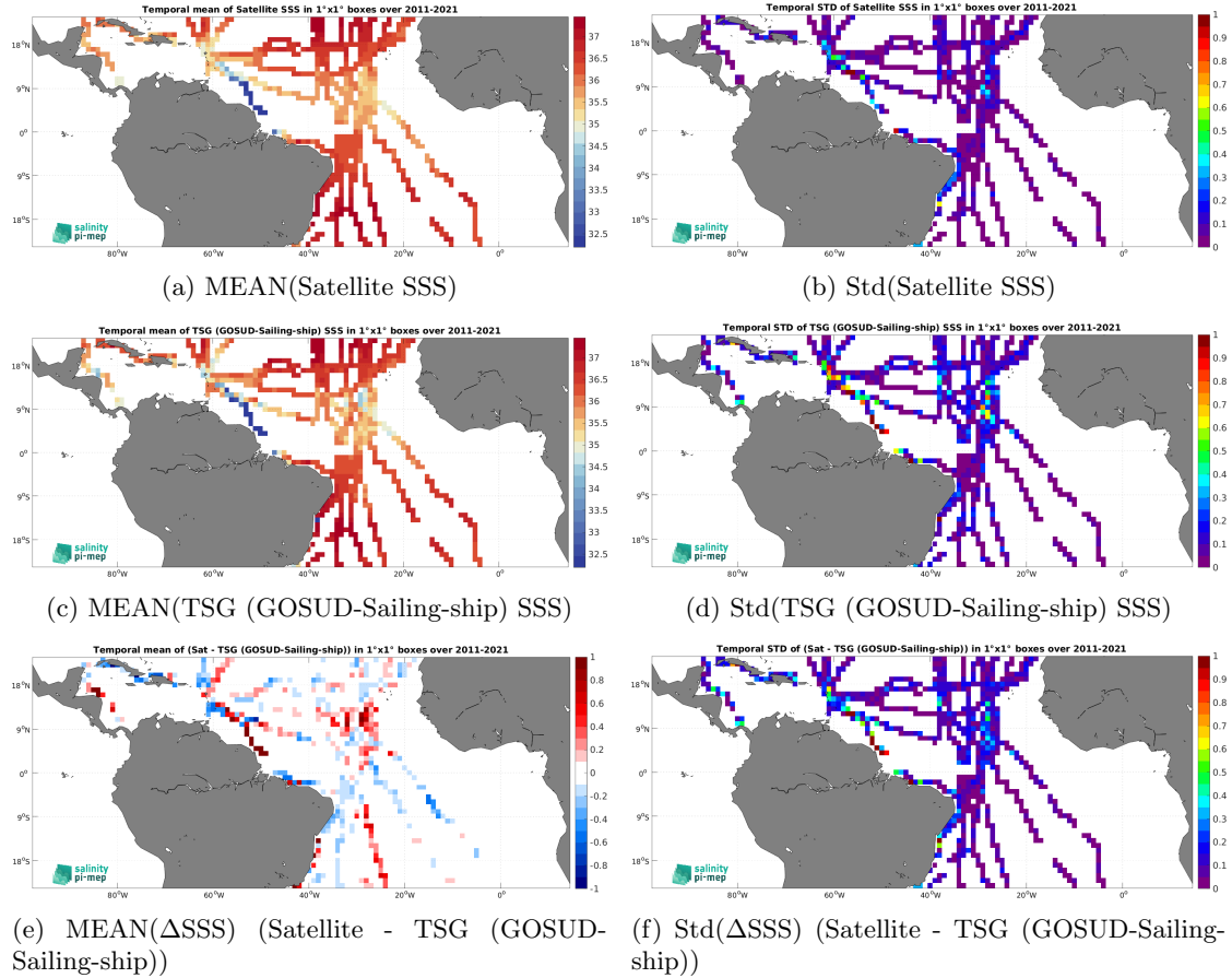
Figure 7: Temporal mean (left) and Std (right) of SSS from SMOS SSS L4 v2 - Daily (BEC) (top), TSG (GOSUD-Sailing-ship) (middle), and of \Delta\text{SSS} (Satellite - TSG (GOSUD-Sailing-ship)). Only match-up pairs are used to generate these maps.
