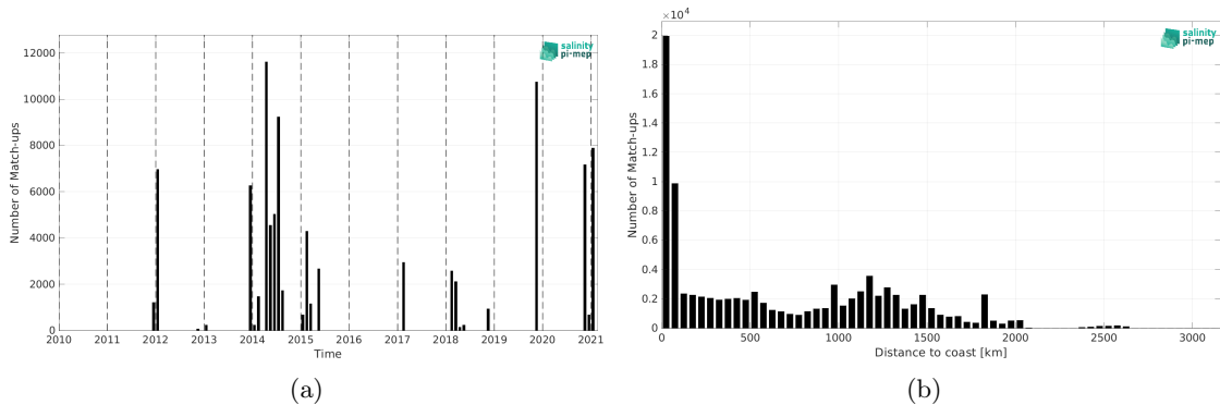
Figure 2: Number of match-ups between TSG (GOSUD-Sailing-ship) and SMOS SSS L4 v2 - Daily (BEC) SSS as a function of time (a) and as function of the distance to coast (b) over the Tropical Atlantic Ocean Pi-MEP region and for the full satellite product period.
