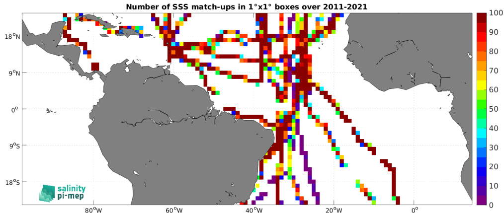
Figure 5: Number of SSS match-ups between TSG (GOSUD-Sailing-ship) SSS and the SMOS SSS L4 v2 - Daily (BEC) SSS product for the Tropical Atlantic Ocean Pi-MEP region over 1^\circ \times 1^\circ boxes and for the full satellite product period.
