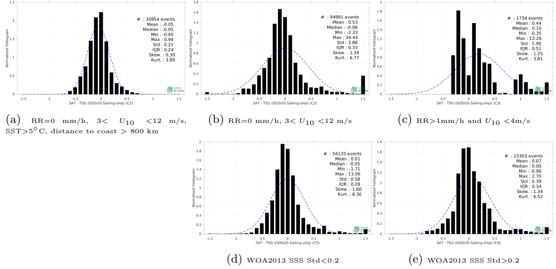
Figure 13: Normalized histogram of \Delta SSS (SMOS SSS L4 v2 - Daily (BEC) - TSG (GOSUD-Sailing-ship)) for 5 different subdatasets corresponding to: RR=0 mm/h, 3 < U_{10} < 12 m/s, SST > 5°C, distance to coast > 800 km (a), RR=0 mm/h, 3 < U_{10} < 12 m/s (b), RR > 1mm/h and U_{10} < 4 m/s (c), WOA2013 SSS Std < 0.2 (d), WOA2013 SSS Std > 0.2 (e).
