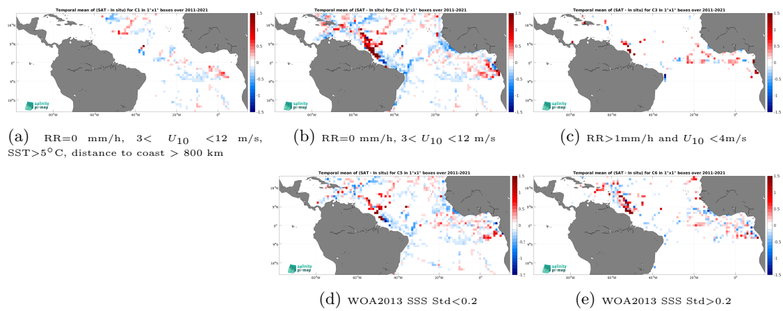
Figure 14: Temporal mean gridded over spatial boxes of size 1^\circ \times 1^\circ of \Delta\text{SSS} (SMOS SSS L4 v2 - Daily (BEC) - TSG (GOSUD-Research-vessel)) for 5 different subdatasets corresponding to:RR=0 mm/h, 3 < U_{10} < 12 m/s, SST>5°C, distance to coast > 800 km (a), RR=0 mm/h, 3 < U_{10} < 12 m/s (b), RR>1mm/h and U_{10} < 4 m/s (c), WOA2013 SSS Std<0.2 (d), WOA2013 SSS Std>0.2 (e).
