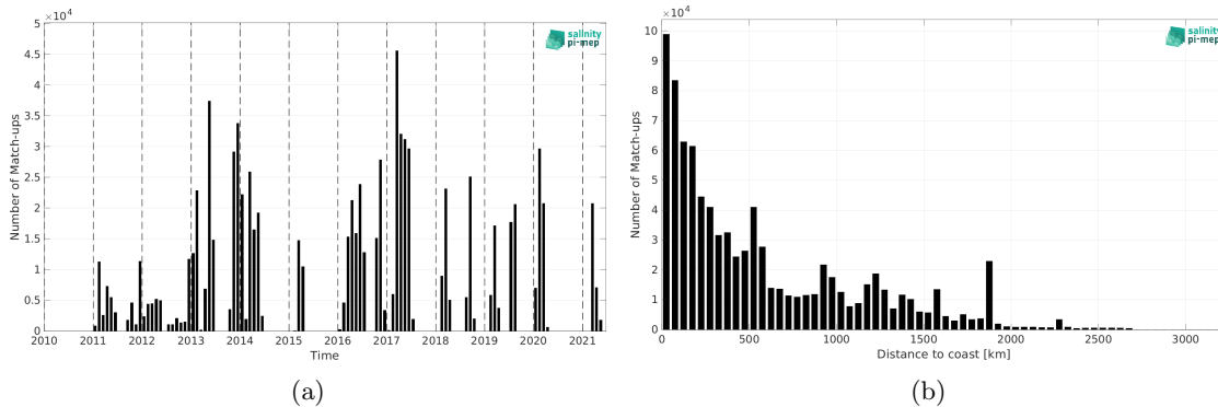
Figure 2: Number of match-ups between TSG (GOSUD-Research-vessel) and SMOS SSS L4 v2 - Daily (BEC) SSS as a function of time (a) and as function of the distance to coast (b) over the Tropical Atlantic Ocean Pi-MEP region and for the full satellite product period.
