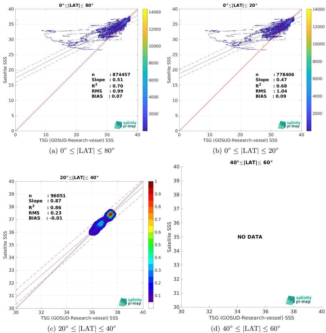
Figure 10: Contour maps of the concentration of SMOS SSS L4 v2 - Daily (BEC) SSS (y-axis) versus TSG (GOSUD-Research-vessel) SSS (x-axis) at match-up pairs for different latitude bands. For each plot, the red line shows x=y . The black thin and dashed lines indicate a linear fit through the data cloud and the \pm 95\% confidence levels, respectively. The number match-up pairs n , the slope and R^2 coefficient of the linear fit, the root mean square (RMS) and the mean bias between satellite and in situ data are indicated for each latitude band in each plots.
