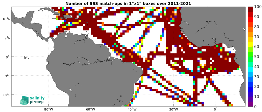
Figure 5: Number of SSS match-ups between TSG (GOSUD-Research-vessel) SSS and the SMOS SSS L4 v2 - Daily (BEC) SSS product for the Tropical Atlantic Ocean Pi-MEP region over 1^\circ \times 1^\circ boxes and for the full satellite product period.
