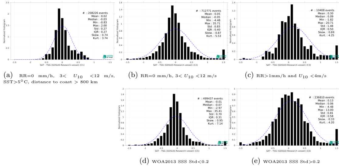
Figure 15: Normalized histogram of \Delta SSS (SMOS SSS L4 v2 - Daily (BEC) - TSG (GOSUD-Research-vessel)) for 5 different subdatasets corresponding to: RR=0 mm/h, 3 < U_{10} < 12 m/s, SST > 5°C, distance to coast > 800 km (a), RR=0 mm/h, 3 < U_{10} < 12 m/s (b), RR > 1mm/h and U_{10} < 4 m/s (c), WOA2013 SSS Std < 0.2 (d), WOA2013 SSS Std > 0.2 (e).
