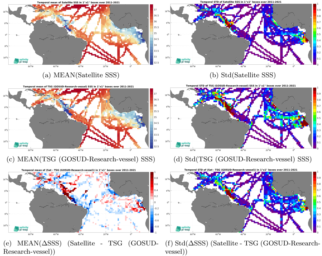
Figure 7: Temporal mean (left) and Std (right) of SSS from SMOS SSS L4 v2 - Daily (BEC) (top), TSG (GOSUD-Research-vessel) (middle), and of \Delta\text{SSS} (Satellite - TSG (GOSUD-Research-vessel)). Only match-up pairs are used to generate these maps.
