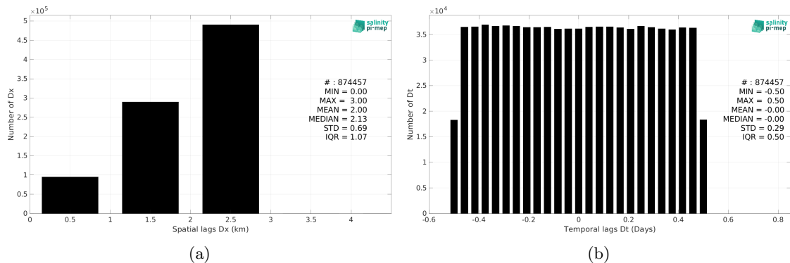
Figure 6: Histograms of the spatial (a) and temporal (b) lags between the location/time of the TSG (GOSUD-Research-vessel) measurement and the date of the corresponding SMOS SSS L4 v2 - Daily (BEC) SSS pixel.
