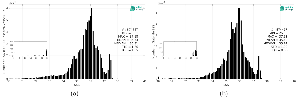
Figure 3: Histograms of SSS from TSG (GOSUD-Research-vessel) (a) and SMOS SSS L4 v2 - Daily (BEC) (b) considering all match-up pairs per bins of 0.1 over the Tropical Atlantic Ocean Pi-MEP region and for the full satellite product period.
