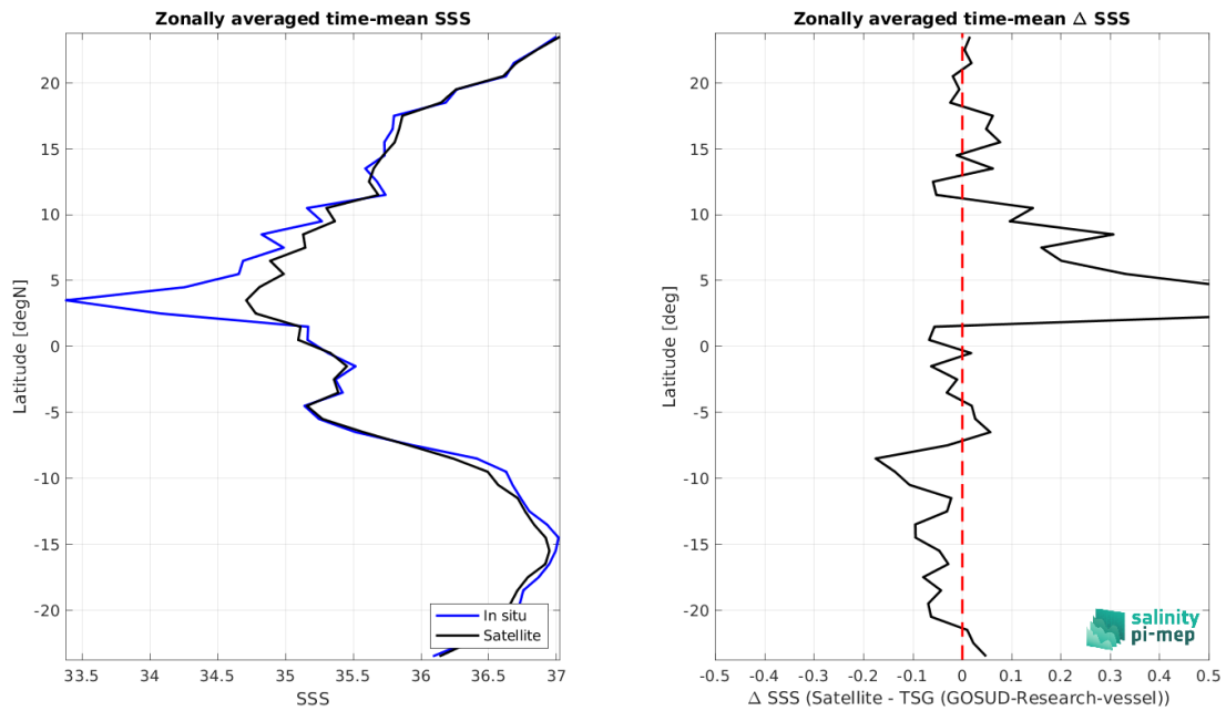
Figure 9: Left panel: Zonal mean SSS from SMOS SSS L4 v2 - Daily (BEC) satellite product (black) and from TSG (GOSUD-Research-vessel) (blue). Right panel: Zonal mean of \Delta SSS (Satellite - TSG (GOSUD-Research-vessel)) for all the collected Pi-MEP match-up pairs estimated over the full satellite product period.
