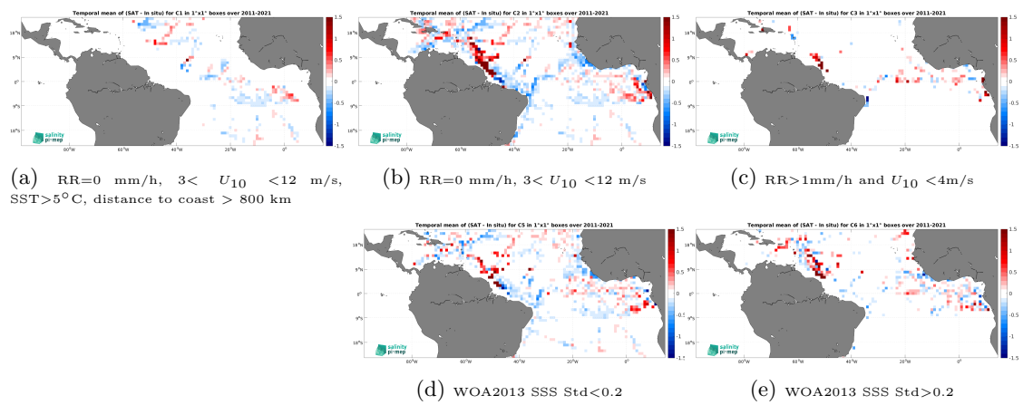
Figure 14: Temporal mean gridded over spatial boxes of size 1^\circ \times 1^\circ of \Delta\text{SSS} (SMOS SSS L4 v2 - Daily (BEC) - TSG (GOSUD-Research-vessel)) for 5 different subdatasets corresponding to:RR=0 mm/h, 3 < U_{10} < 12 m/s, SST>5°C, distance to coast > 800 km (a), RR=0 mm/h, 3 < U_{10} < 12 m/s (b), RR>1mm/h and U_{10} < 4 m/s (c), WOA2013 SSS Std<0.2 (d), WOA2013 SSS Std>0.2 (e).
