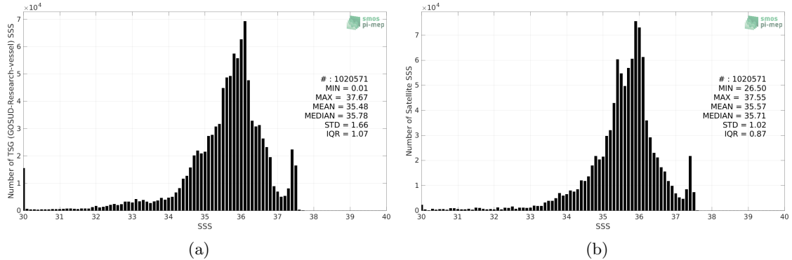
Figure 2: Histograms of SSS from TSG (GOSUD-Research-vessel) (a) and SMOS SSS L4 v2 - Daily (BEC) (b) considering all match-up pairs per bins of 0.1 over the Tropical Atlantic Ocean Pi-MEP region and for the full satellite product period.
