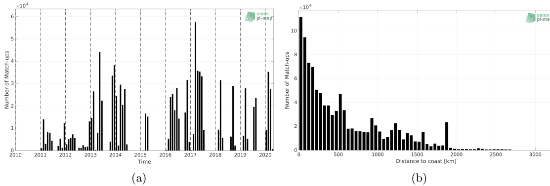
Figure 1: Number of match-ups between TSG (GOSUD-Research-vessel) and SMOS SSS L4 v2 - Daily (BEC) SSS as a function of time (a) and as function of the distance to coast (b) over the Tropical Atlantic Ocean Pi-MEP region and for the full satellite product period.
