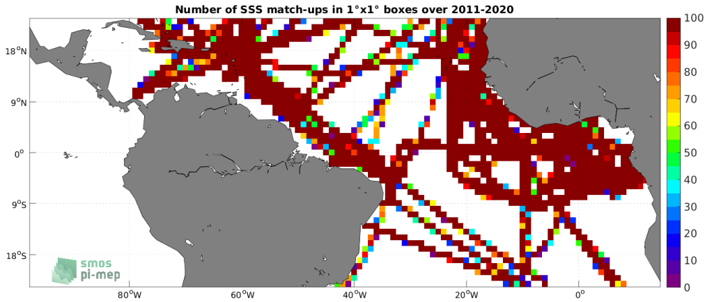
Figure 4: Number of SSS match-ups between TSG (GOSUD-Research-vessel) SSS and the SMOS SSS L4 v2 - Daily (BEC) SSS product for the Tropical Atlantic Ocean Pi-MEP region over 1^\circ \times 1^\circ boxes and for the full satellite product period.
