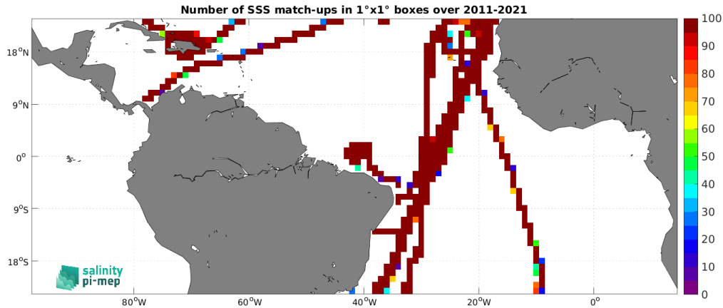
Figure 5: Number of SSS match-ups between TSG (CSIC-UTM) SSS and the SMOS SSS L4 v2 - Daily (BEC) SSS product for the Tropical Atlantic Ocean Pi-MEP region over 1^\circ \times 1^\circ boxes and for the full satellite product period.
