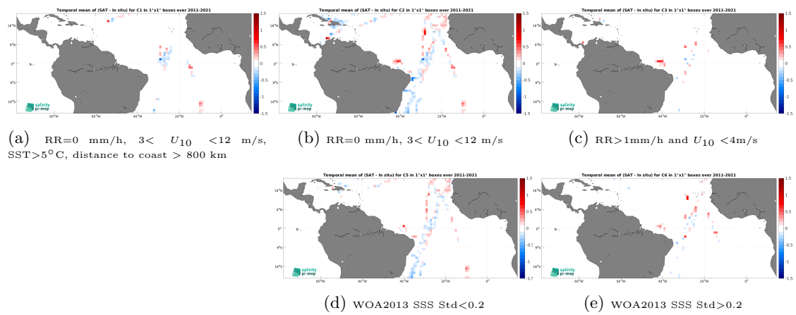
Figure 14: Temporal mean gridded over spatial boxes of size 1^\circ \times 1^\circ of \Delta\text{SSS} (SMOS SSS L4 v2 - Daily (BEC) - TSG (CSIC-UTM)) for 5 different subdatasets corresponding to:RR=0 mm/h, 3 < U_{10} < 12 m/s, SST >5^\circ\text{C} , distance to coast > 800 km (a), RR=0 mm/h, 3 < U_{10} < 12 m/s (b), RR >1 mm/h and U_{10} < 4 m/s (c), WOA2013 SSS Std <0.2 (d), WOA2013 SSS Std >0.2 (e).
