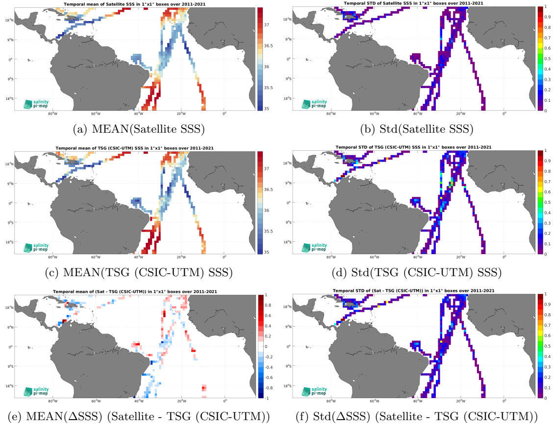
Figure 7: Temporal mean (left) and Std (right) of SSS from SMOS SSS L4 v2 - Daily (BEC) (top), TSG (CSIC-UTM) (middle), and of \Delta\text{SSS} (Satellite - TSG (CSIC-UTM)). Only match-up pairs are used to generate these maps.
