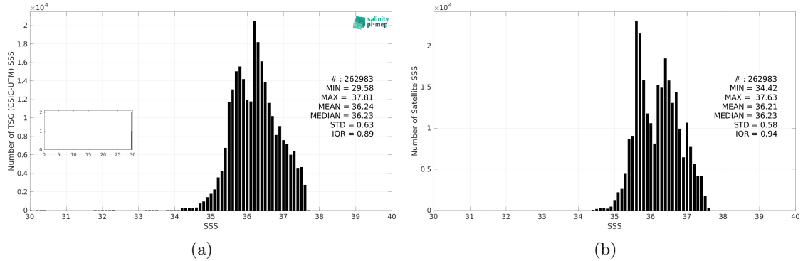
Figure 3: Histograms of SSS from TSG (CSIC-UTM) (a) and SMOS SSS L4 v2 - Daily (BEC) (b) considering all match-up pairs per bins of 0.1 over the Tropical Atlantic Ocean Pi-MEP region and for the full satellite product period.
