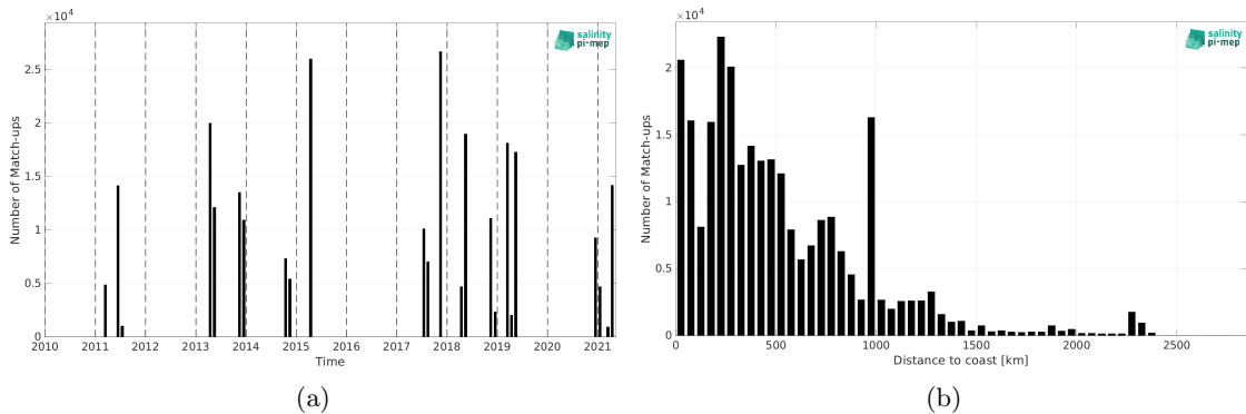
Figure 2: Number of match-ups between TSG (CSIC-UTM) and SMOS SSS L4 v2 - Daily (BEC) SSS as a function of time (a) and as function of the distance to coast (b) over the Tropical Atlantic Ocean Pi-MEP region and for the full satellite product period.
