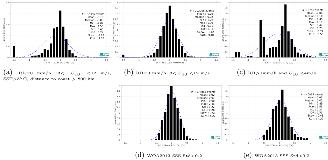
Figure 15: Normalized histogram of \Delta\text{SSS} (SMOS SSS L4 v2 - Daily (BEC) - TSG (CSIC-UTM)) for 5 different subdatasets corresponding to: RR=0 mm/h, 3 < U_{10} < 12 m/s, SST > 5^\circ\text{C} , distance to coast > 800 km (a), RR=0 mm/h, 3 < U_{10} < 12 m/s (b), RR > 1 mm/h and U_{10} < 4 m/s (c), WOA2013 SSS Std < 0.2 (d), WOA2013 SSS Std > 0.2 (e).
