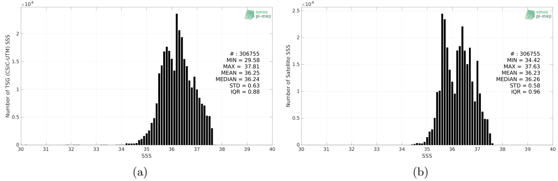
Figure 2: Histograms of SSS from TSG (CSIC-UTM) (a) and SMOS SSS L4 v2 - Daily (BEC) (b) considering all match-up pairs per bins of 0.1 over the Tropical Atlantic Ocean Pi-MEP region and for the full satellite product period.
