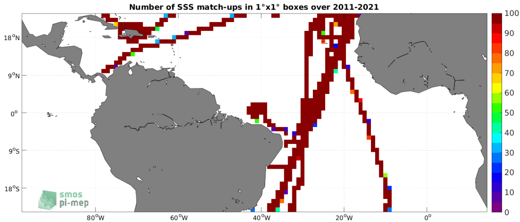
Figure 4: Number of SSS match-ups between TSG (CSIC-UTM) SSS and the SMOS SSS L4 v2 - Daily (BEC) SSS product for the Tropical Atlantic Ocean Pi-MEP region over 1^\circ \times 1^\circ boxes and for the full satellite product period.
