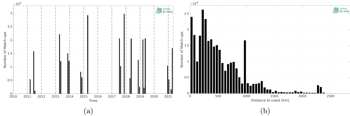
Figure 1: Number of match-ups between TSG (CSIC-UTM) and SMOS SSS L4 v2 - Daily (BEC) SSS as a function of time (a) and as function of the distance to coast (b) over the Tropical Atlantic Ocean Pi-MEP region and for the full satellite product period.
