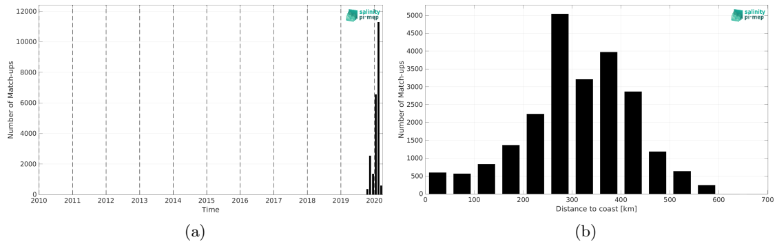
Figure 2: Number of match-ups between Sairdrone and SMOS SSS L4 v2 - Daily (BEC) SSS as a function of time (a) and as function of the distance to coast (b) over the Tropical Atlantic Ocean Pi-MEP region and for the full satellite product period.
