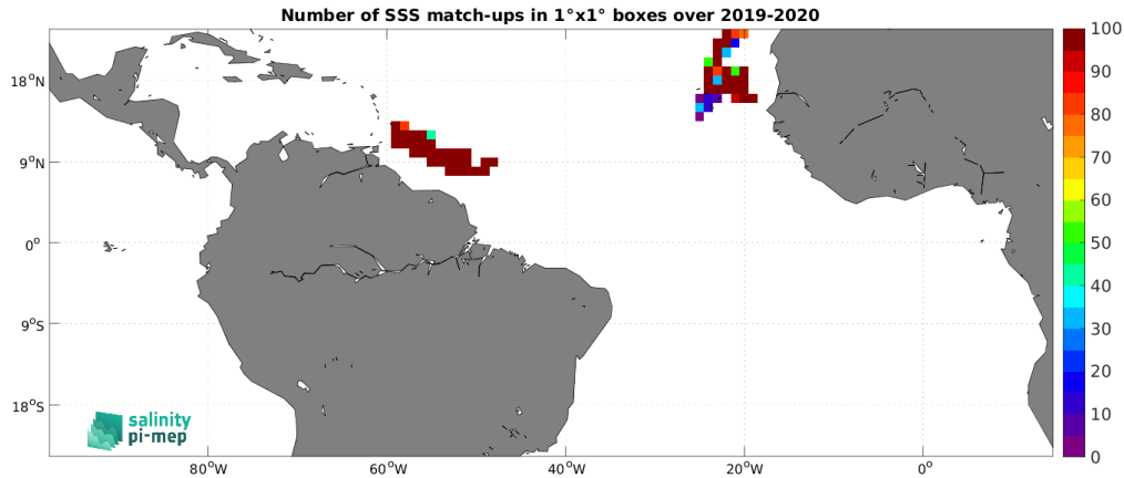
Figure 5: Number of SSS match-ups between Saildrone SSS and the SMOS SSS L4 v2 - Daily (BEC) SSS product for the Tropical Atlantic Ocean Pi-MEP region over 1^\circ \times 1^\circ boxes and for the full satellite product period.
