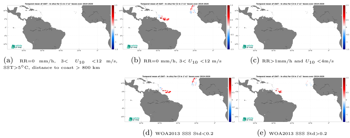
Figure 14: Temporal mean gridded over spatial boxes of size 1^\circ \times 1^\circ of \Delta\text{SSS} (SMOS SSS L4 v2 - Daily (BEC) - Saldrone) for 5 different subdatasets corresponding to:RR=0 mm/h, 3 < U_{10} < 12 m/s, SST>5°C, distance to coast > 800 km (a), RR=0 mm/h, 3 < U_{10} < 12 m/s (b), RR>1mm/h and U_{10} < 4 m/s (c), WOA2013 SSS Std<0.2 (d), WOA2013 SSS Std>0.2 (e).
