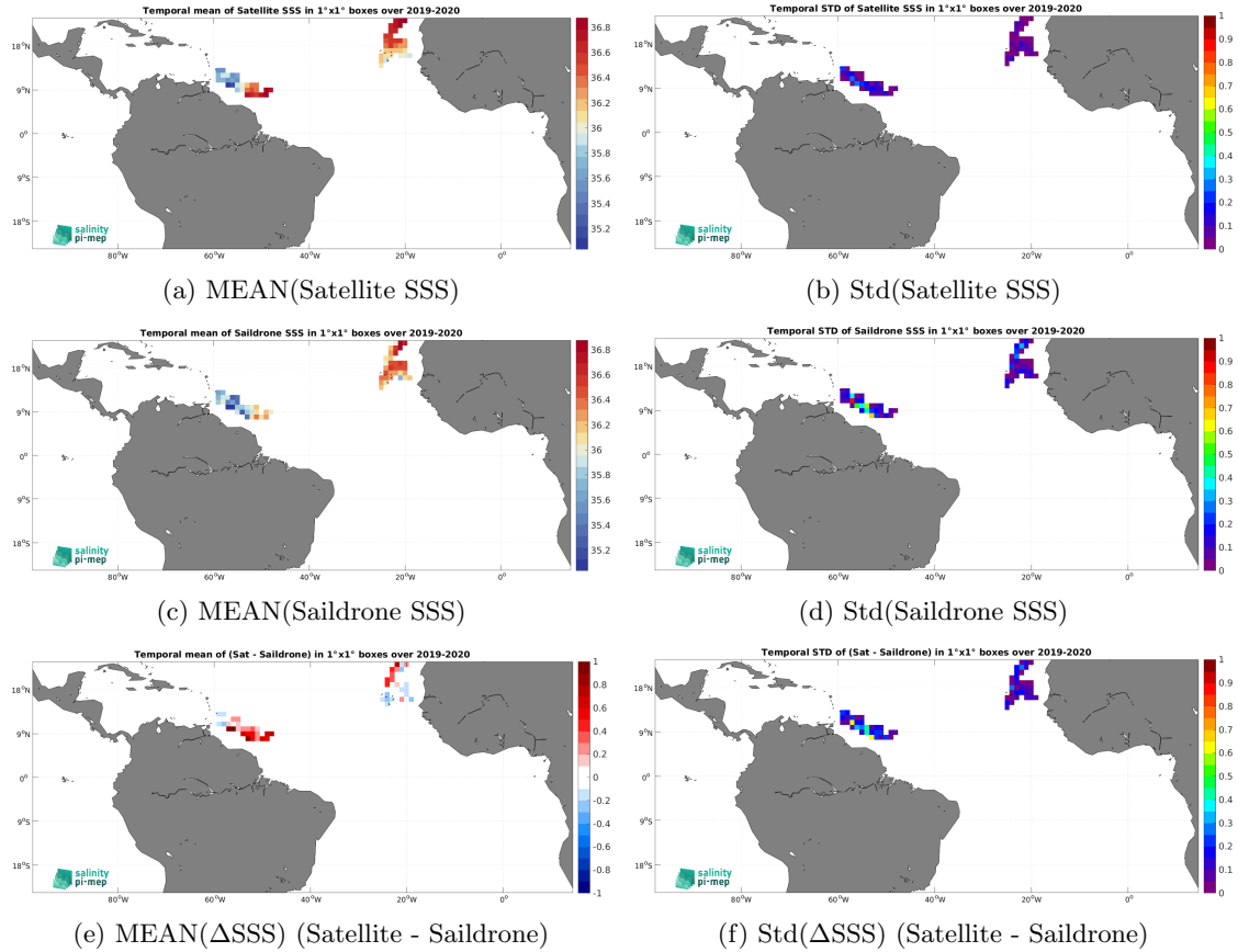
Figure 7: Temporal mean (left) and Std (right) of SSS from SMOS SSS L4 v2 - Daily (BEC) (top), Sairdron (middle), and of \Delta SSS (Satellite - Sairdron). Only match-up pairs are used to generate these maps.
