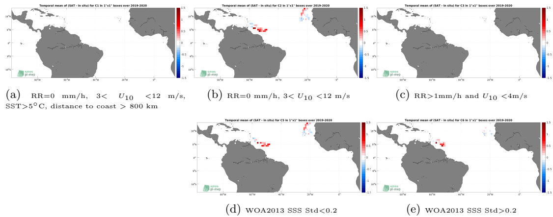
Figure 12: Temporal mean gridded over spatial boxes of size 1^\circ \times 1^\circ of \Delta\text{SSS} (SMOS SSS L4 v2 - Daily (BEC) - Sairdrone) for 5 different subdatasets corresponding to:RR=0 mm/h, 3 < U_{10} < 12 m/s, SST >5^\circ\text{C} , distance to coast > 800 km (a), RR=0 mm/h, 3 < U_{10} < 12 m/s (b), RR >1 mm/h and U_{10} < 4 m/s (c), WOA2013 SSS Std <0.2 (d), WOA2013 SSS Std >0.2 (e).
