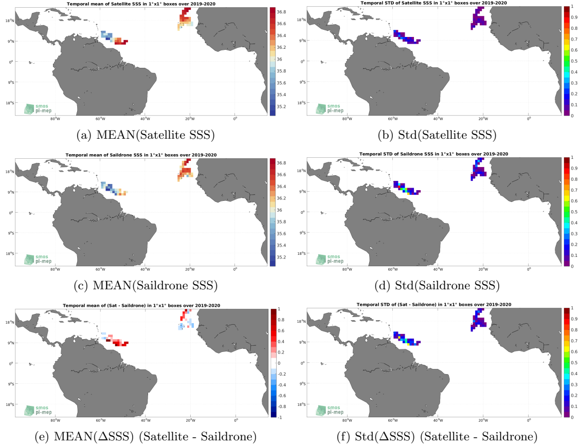
Figure 6: Temporal mean (left) and Std (right) of SSS from SMOS SSS L4 v2 - Daily (BEC) (top), Sairdrone (middle), and of \Delta SSS (Satellite - Sairdrone). Only match-up pairs are used to generate these maps.
