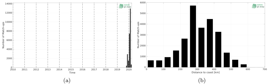
Figure 1: Number of match-ups between Sairdrone and SMOS SSS L4 v2 - Daily (BEC) SSS as a function of time (a) and as function of the distance to coast (b) over the Tropical Atlantic Ocean Pi-MEP region and for the full satellite product period.
