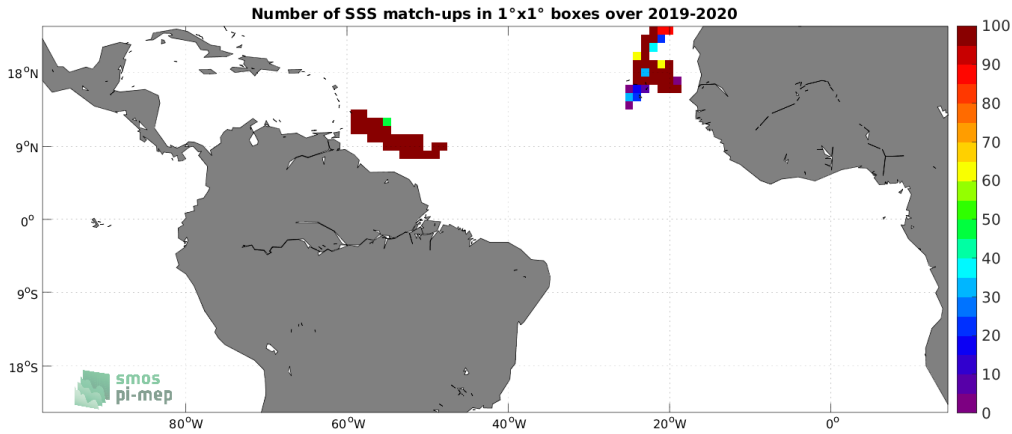
Figure 4: Number of SSS match-ups between Saildrone SSS and the SMOS SSS L4 v2 - Daily (BEC) SSS product for the Tropical Atlantic Ocean Pi-MEP region over 1^\circ \times 1^\circ boxes and for the full satellite product period.
