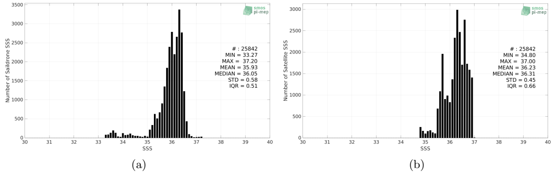
Figure 2: Histograms of SSS from Sairdrone (a) and SMOS SSS L4 v2 - Daily (BEC) (b) considering all match-up pairs per bins of 0.1 over the Tropical Atlantic Ocean Pi-MEP region and for the full satellite product period.
