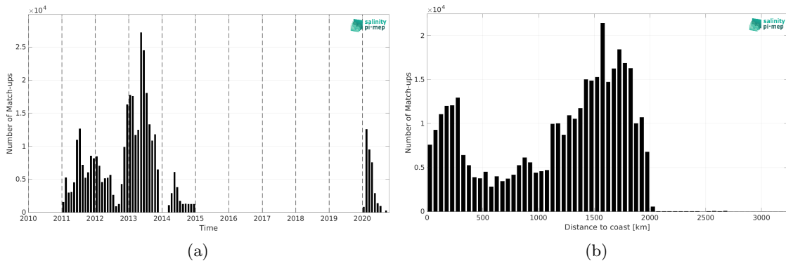
Figure 2: Number of match-ups between Surface drifters and SMOS SSS L4 v2 - Daily (BEC) SSS as a function of time (a) and as function of the distance to coast (b) over the Tropical Atlantic Ocean Pi-MEP region and for the full satellite product period.
