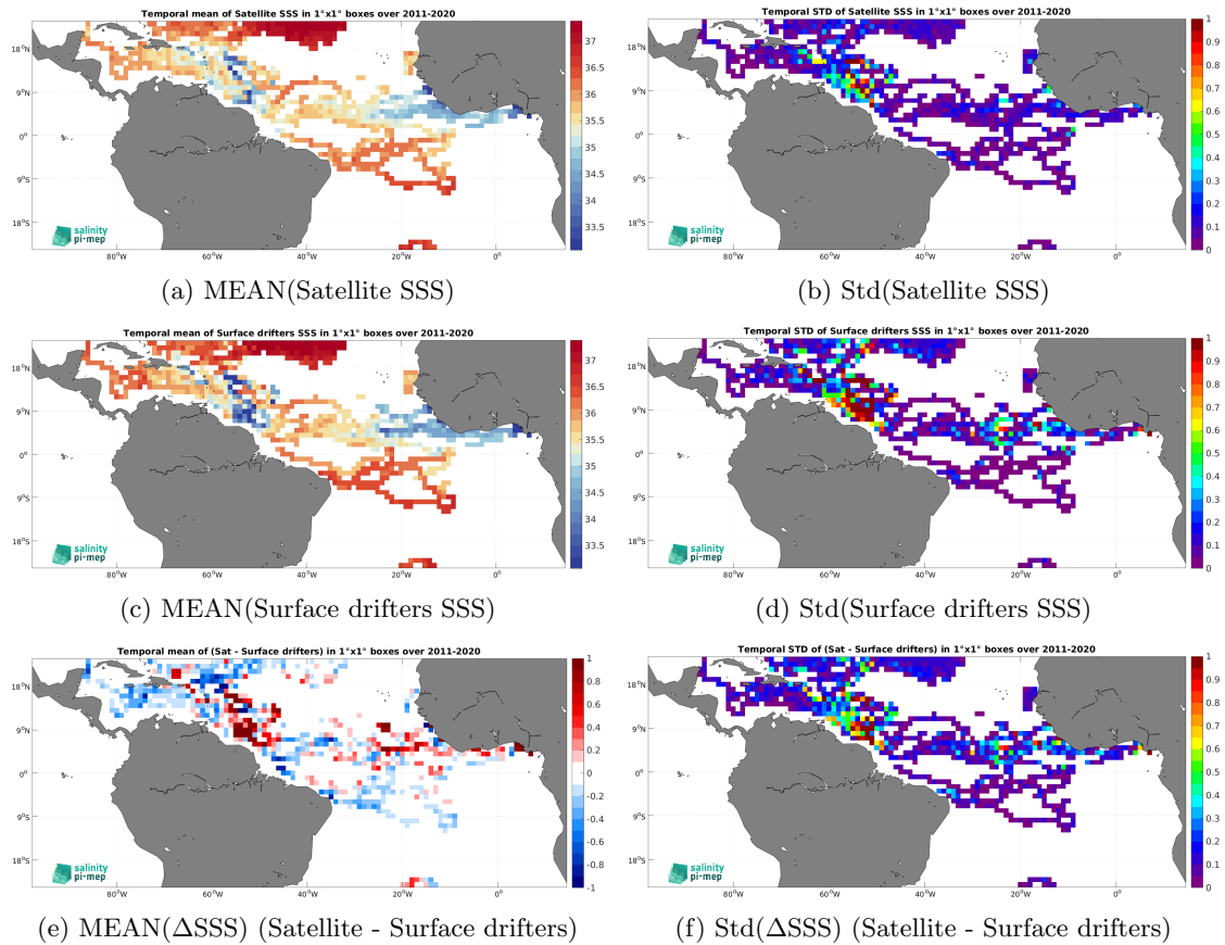
Figure 6: Temporal mean (left) and Std (right) of SSS from SMOS SSS L4 v2 - Daily (BEC) (top), Surface drifters (middle), and of \Delta SSS (Satellite - Surface drifters). Only match-up pairs are used to generate these maps.
