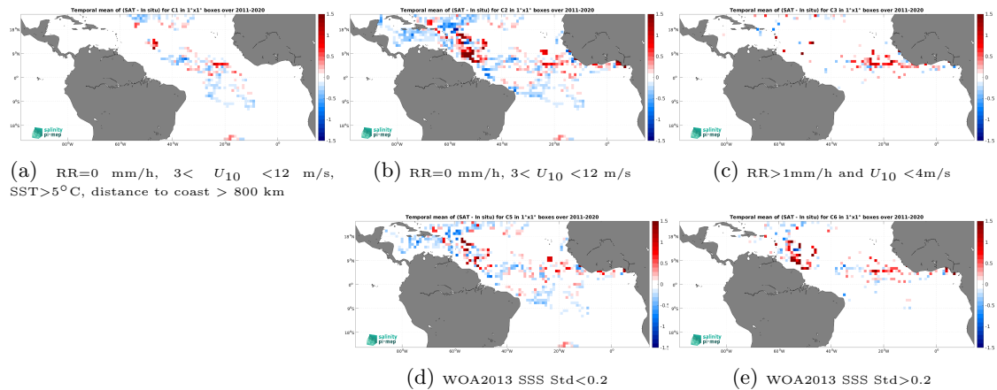
Figure 13: Temporal mean gridded over spatial boxes of size 1^\circ \times 1^\circ of \Delta\text{SSS} (SMOS SSS L4 v2 - Daily (BEC) - Surface drifters) for 5 different subdatasets corresponding to:RR=0 mm/h, 3 < U_{10} < 12 m/s, SST >5^\circ\text{C} , distance to coast > 800 km (a), RR=0 mm/h, 3 < U_{10} < 12 m/s (b), RR >1 mm/h and U_{10} < 4 m/s (c), WOA2013 SSS Std <0.2 (d), WOA2013 SSS Std >0.2 (e).
