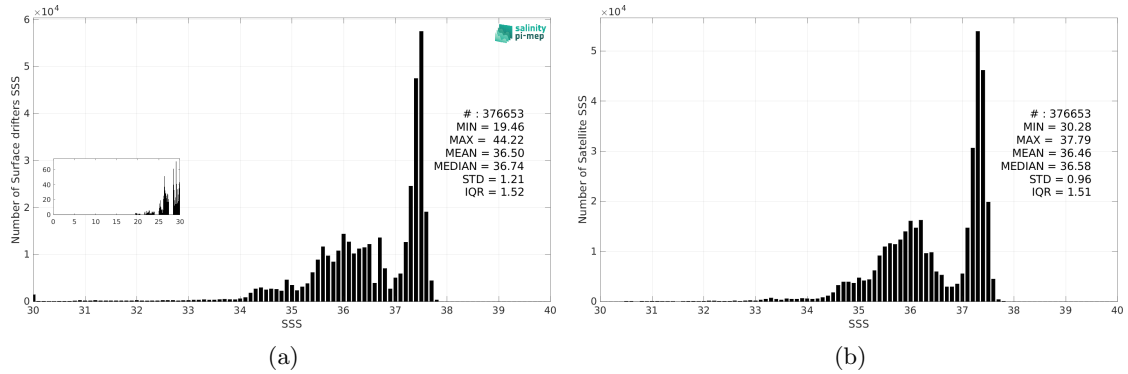
Figure 3: Histograms of SSS from Surface drifters (a) and SMOS SSS L4 v2 - Daily (BEC) (b) considering all match-up pairs per bins of 0.1 over the Tropical Atlantic Ocean Pi-MEP region and for the full satellite product period.
