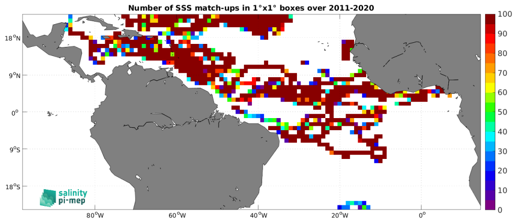
Figure 4: Number of SSS match-ups between Surface drifters SSS and the SMOS SSS L4 v2 - Daily (BEC) SSS product for the Tropical Atlantic Ocean Pi-MEP region over 1^\circ \times 1^\circ boxes and for the full satellite product period.
