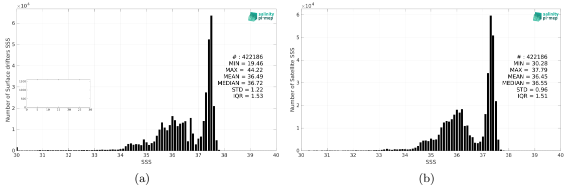
Figure 2: Histograms of SSS from Surface drifters (a) and SMOS SSS L4 v2 - Daily (BEC) (b) considering all match-up pairs per bins of 0.1 over the Tropical Atlantic Ocean Pi-MEP region and for the full satellite product period.
