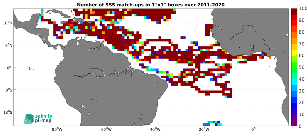
Figure 3: Number of SSS match-ups between Surface drifters SSS and the SMOS SSS L4 v2 - Daily (BEC) SSS product for the Tropical Atlantic Ocean Pi-MEP region over 1^\circ \times 1^\circ boxes and for the full satellite product period.
