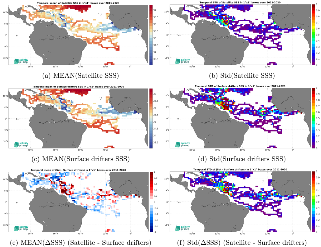
Figure 5: Temporal mean (left) and Std (right) of SSS from SMOS SSS L4 v2 - Daily (BEC) (top), Surface drifters (middle), and of \Delta SSS (Satellite - Surface drifters). Only match-up pairs are used to generate these maps.
