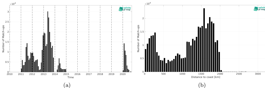
Figure 1: Number of match-ups between Surface drifters and SMOS SSS L4 v2 - Daily (BEC) SSS as a function of time (a) and as function of the distance to coast (b) over the Tropical Atlantic Ocean Pi-MEP region and for the full satellite product period.
