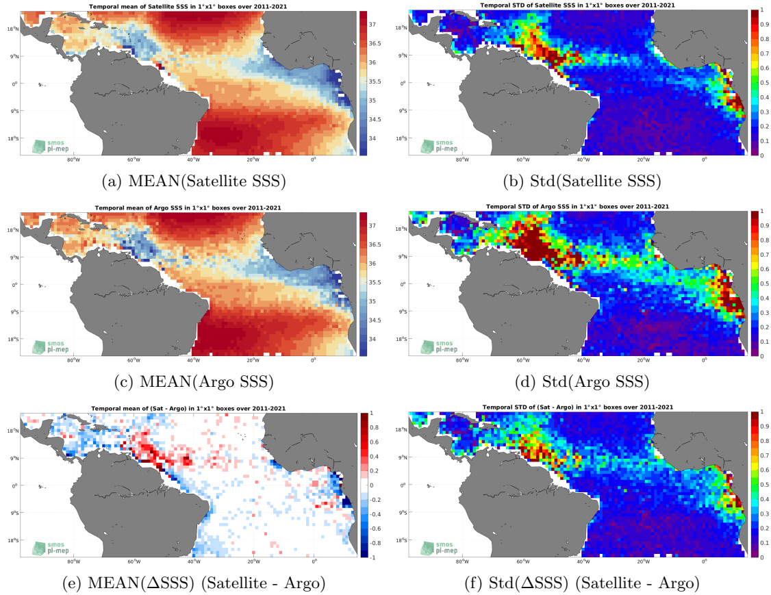
Figure 6: Temporal mean (left) and Std (right) of SSS from SMOS SSS L4 v2 - Daily (BEC) (top), Argo (middle), and of \Delta SSS (Satellite - Argo). Only match-up pairs are used to generate these maps.
