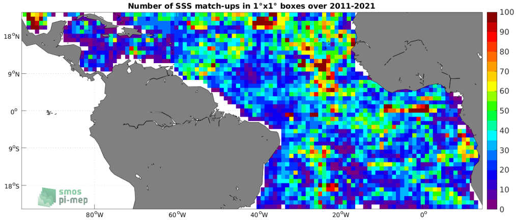
Figure 4: Number of SSS match-ups between Argo SSS and the SMOS SSS L4 v2 - Daily (BEC) SSS product for the Tropical Atlantic Ocean Pi-MEP region over 1^\circ \times 1^\circ boxes and for the full satellite product period.
