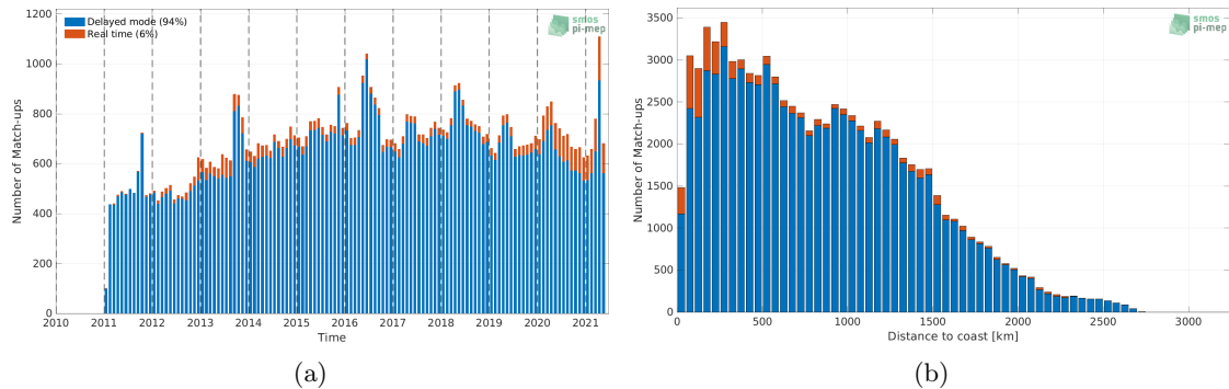
Figure 1: Number of match-ups between Argo and SMOS SSS L4 v2 - Daily (BEC) SSS as a function of time (a) and as function of the distance to coast (b) over the Tropical Atlantic Ocean Pi-MEP region and for the full satellite product period.
