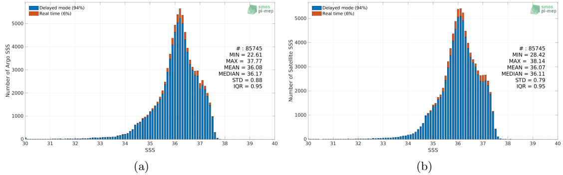
Figure 2: Histograms of SSS from Argo (a) and SMOS SSS L4 v2 - Daily (BEC) (b) considering all match-up pairs per bins of 0.1 over the Tropical Atlantic Ocean Pi-MEP region and for the full satellite product period.
