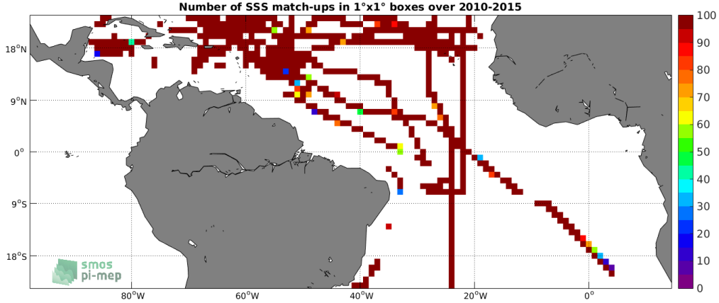
Figure 4: Number of SSS match-ups between TSG (SAMOS) SSS and the SMOS SSS L3 v3 Monthly (ICDC) SSS product for the Tropical Atlantic Ocean Pi-MEP region over 1^\circ \times 1^\circ boxes and for the full satellite product period.
