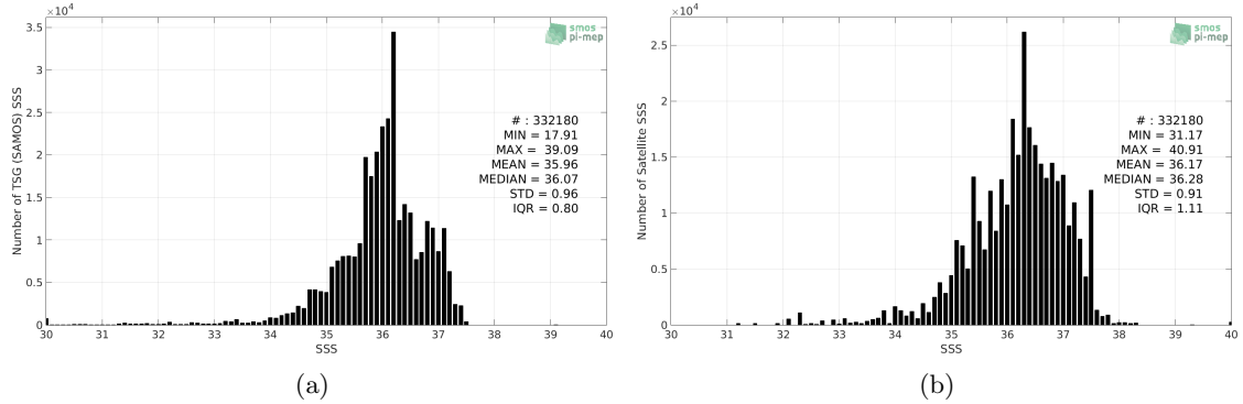
Figure 2: Histograms of SSS from TSG (SAMOS) (a) and SMOS SSS L3 v3 Monthly (ICDC) (b) considering all match-up pairs per bins of 0.1 over the Tropical Atlantic Ocean Pi-MEP region and for the full satellite product period.
