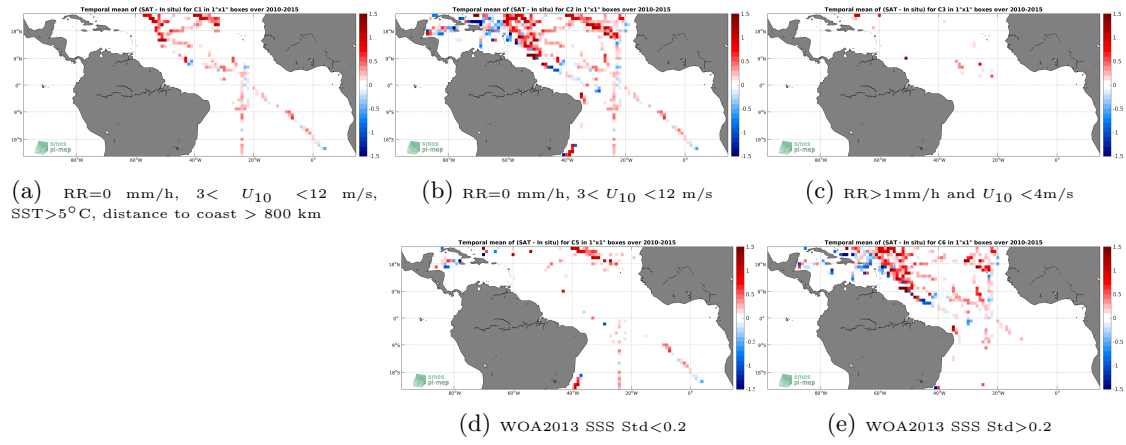
Figure 12: Temporal mean gridded over spatial boxes of size 1^\circ \times 1^\circ of \Delta SSS (SMOS SSS L3 v3 Monthly (ICDC) - TSG (SAMOS)) for 5 different subdatasets corresponding to:RR=0 mm/h, 3 < U_{10} < 12 m/s, SST >5^\circ\text{C} , distance to coast > 800 km (a), RR=0 mm/h, 3 < U_{10} < 12 m/s (b), RR >1 mm/h and U_{10} < 4 m/s (c), WOA2013 SSS Std <0.2 (d), WOA2013 SSS Std >0.2 (e).
