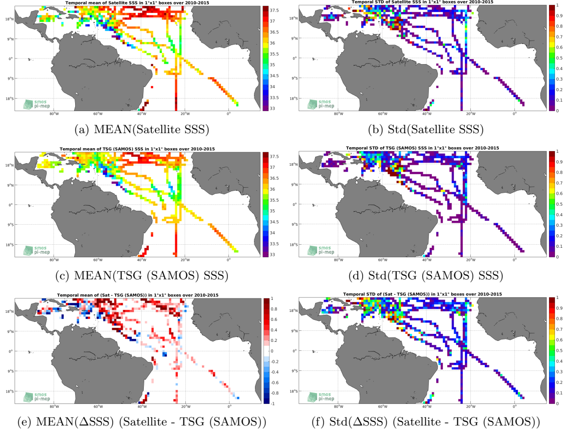
Figure 6: Temporal mean (left) and Std (right) of SSS from SMOS SSS L3 v3 Monthly (ICDC) (top), TSG (SAMOS) (middle), and of \Delta\text{SSS} (Satellite - TSG (SAMOS)). Only match-up pairs are used to generate these maps.
