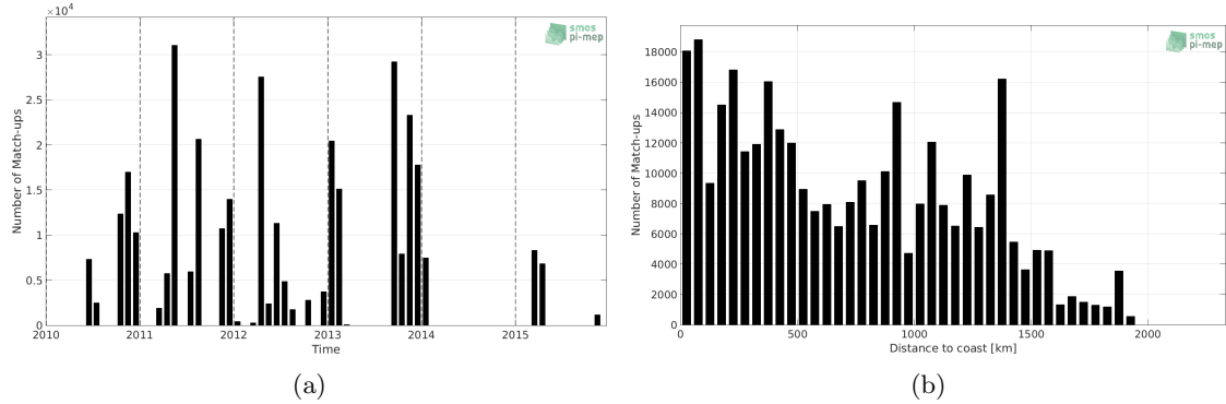
Figure 1: Number of match-ups between TSG (SAMOS) and SMOS SSS L3 v3 Monthly (ICDC) SSS as a function of time (a) and as function of the distance to coast (b) over the Tropical Atlantic Ocean Pi-MEP region and for the full satellite product period.
