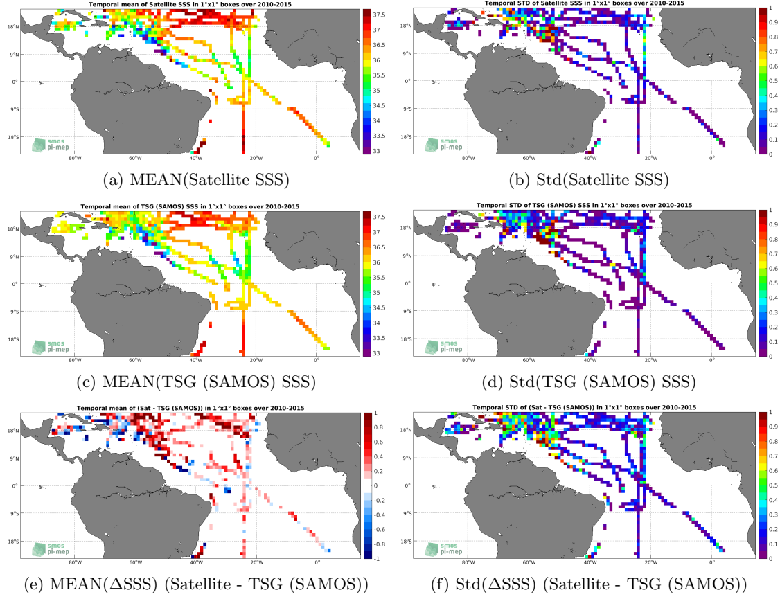
Figure 6: Temporal mean (left) and Std (right) of SSS from SMOS SSS L3 v3 Monthly (ICDC) (top), TSG (SAMOS) (middle), and of \Delta SSS (Satellite - TSG (SAMOS)). Only match-up pairs are used to generate these maps.
