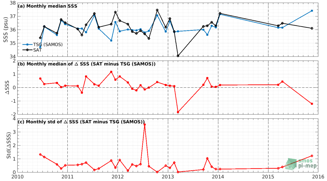
Figure 7: Time series of the monthly median SSS (top), median of \Delta\text{SSS} (Satellite - TSG (SAMOS)) and Std of \Delta\text{SSS} (Satellite - TSG (SAMOS)) over the Tropical Atlantic Ocean Pi-MEP region considering all match-ups collected by the Pi-MEP.
