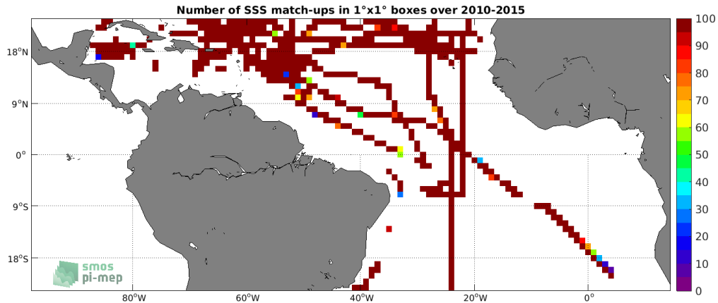
Figure 4: Number of SSS match-ups between TSG (SAMOS) SSS and the SMOS SSS L3 v3 Monthly (ICDC) SSS product for the Tropical Atlantic Ocean Pi-MEP region over 1°x1° boxes and for the full satellite product period.
