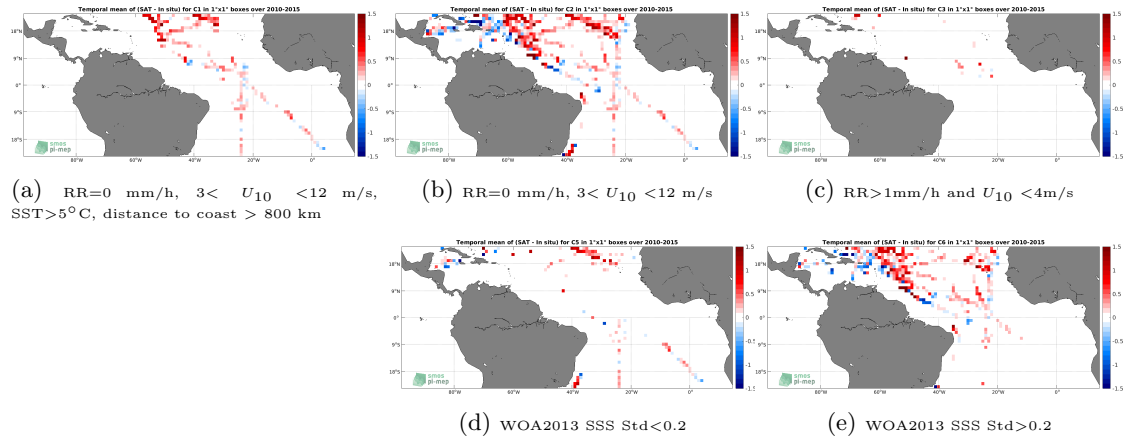
Figure 12: Temporal mean gridded over spatial boxes of size 1^\circ \times 1^\circ of \Delta SSS (SMOS SSS L3 v3 Monthly (ICDC) - TSG (SAMOS)) for 5 different subdatasets corresponding to: RR=0 mm/h, 3 < U_{10} < 12 m/s, SST > 5^\circ\text{C} , distance to coast > 800 km (a), RR=0 mm/h, 3 < U_{10} < 12 m/s (b), RR > 1 mm/h and U_{10} < 4 m/s (c), WOA2013 SSS Std < 0.2 (d), WOA2013 SSS Std > 0.2 (e).
