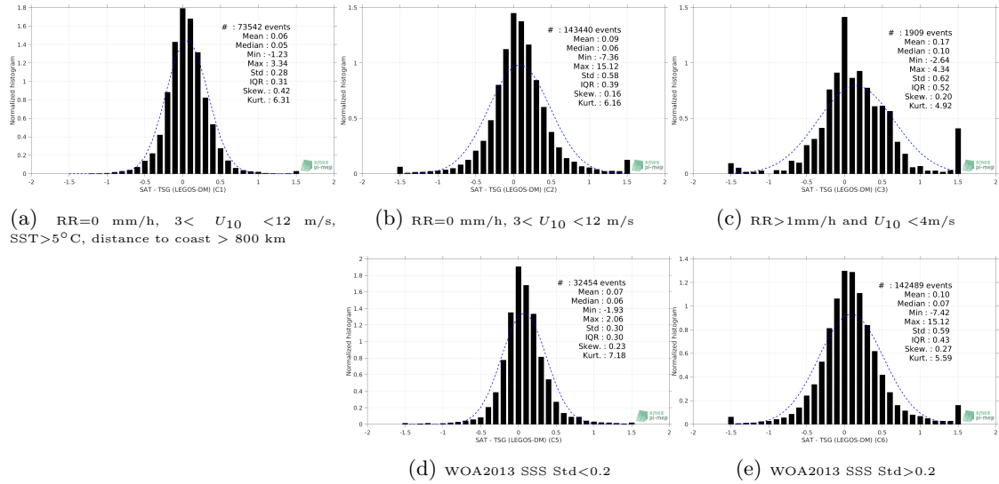
Figure 13: Normalized histogram of \Delta SSS (SMOS SSS L3 v3 Monthly (ICDC) - TSG (LEGOS-DMI)) for 5 different subdatasets corresponding to: RR=0 mm/h, 3 < U_{10} < 12 m/s, SST > 5°C, distance to coast > 800 km (a), RR=0 mm/h, 3 < U_{10} < 12 m/s (b), RR > 1mm/h and U_{10} < 4 m/s (c), WOA2013 SSS Std < 0.2 (d), WOA2013 SSS Std > 0.2 (e).
