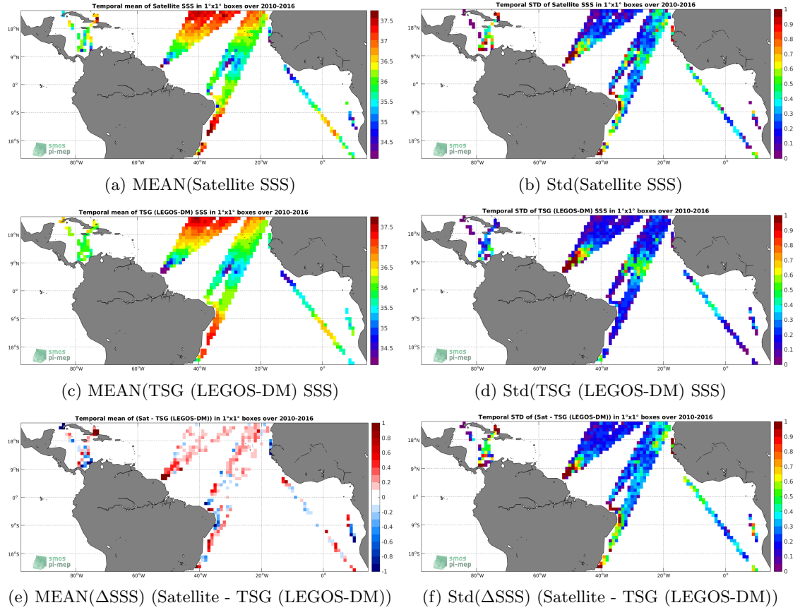
Figure 6: Temporal mean (left) and Std (right) of SSS from SMOS SSS L3 v3 Monthly (ICDC) (top), TSG (LEGOS-DM) (middle), and of \Delta\text{SSS} (Satellite - TSG (LEGOS-DM)). Only match-up pairs are used to generate these maps.
