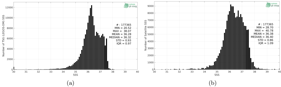
Figure 2: Histograms of SSS from TSG (LEGOS-DM) (a) and SMOS SSS L3 v3 Monthly (ICDC) (b) considering all match-up pairs per bins of 0.1 over the Tropical Atlantic Ocean Pi-MEP region and for the full satellite product period.
