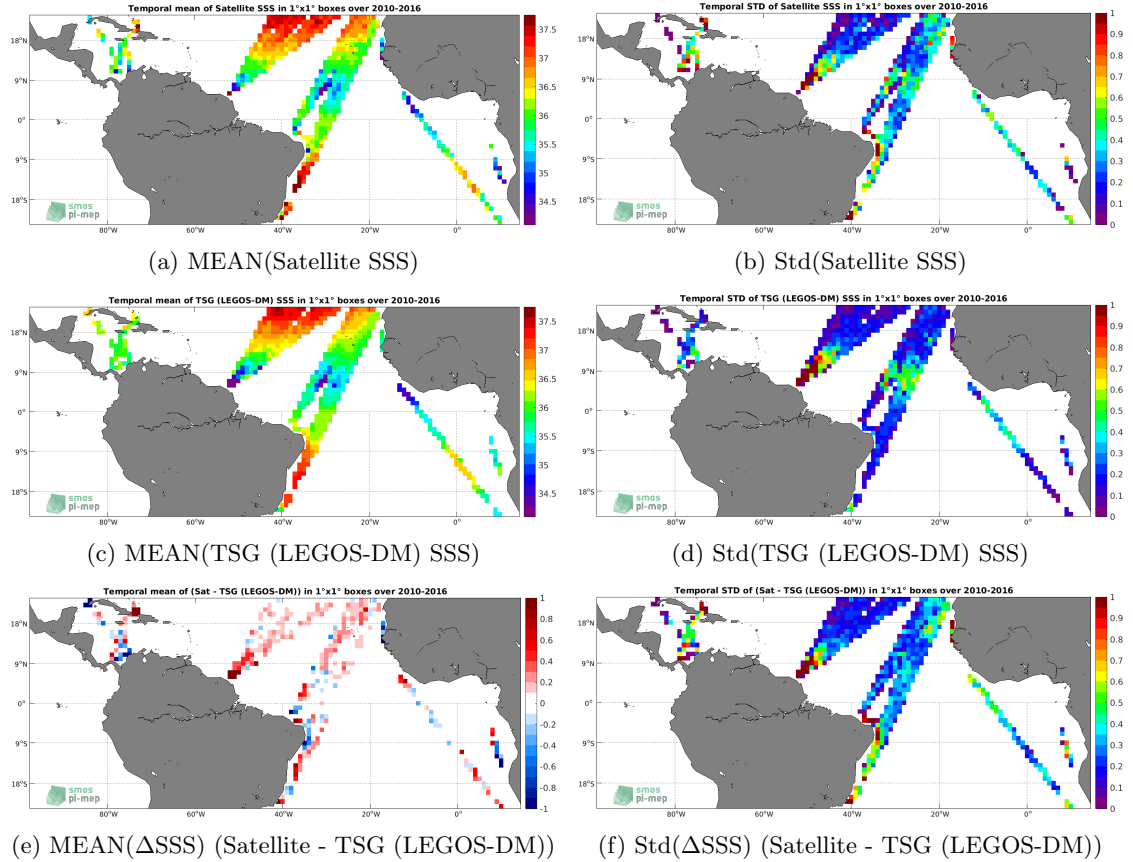
Figure 6: Temporal mean (left) and Std (right) of SSS from SMOS SSS L3 v3 Monthly (ICDC) (top), TSG (LEGOS-DM) (middle), and of \Delta SSS (Satellite - TSG (LEGOS-DM)). Only match-up pairs are used to generate these maps.
