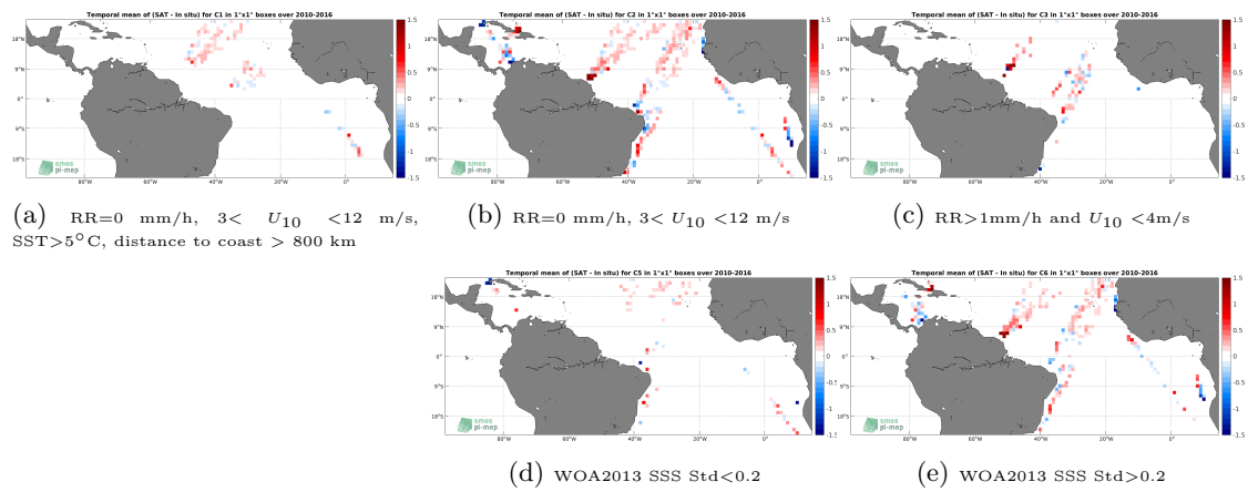
Figure 12: Temporal mean gridded over spatial boxes of size 1^\circ \times 1^\circ of \Delta SSS (SMOS SSS L3 v3 Monthly (ICDC) - TSG (LEGOS-DM)) for 5 different subdatasets corresponding to:RR=0 mm/h, 3 < U_{10} < 12 m/s, SST >5^\circ\text{C} , distance to coast > 800 km (a), RR=0 mm/h, 3 < U_{10} < 12 m/s (b), RR >1 mm/h and U_{10} < 4 m/s (c), WOA2013 SSS Std <0.2 (d), WOA2013 SSS Std >0.2 (e).
