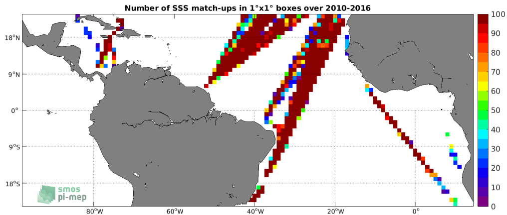
Figure 4: Number of SSS match-ups between TSG (LEGOS-DM) SSS and the SMOS SSS L3 v3 Monthly (ICDC) SSS product for the Tropical Atlantic Ocean Pi-MEP region over 1^\circ \times 1^\circ boxes and for the full satellite product period.
