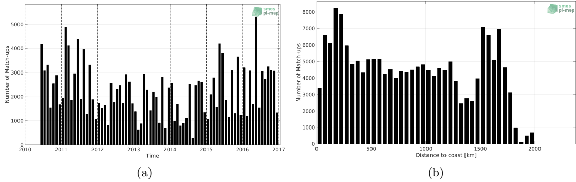
Figure 1: Number of match-ups between TSG (LEGOS-DM) and SMOS SSS L3 v3 Monthly (ICDC) SSS as a function of time (a) and as function of the distance to coast (b) over the Tropical Atlantic Ocean Pi-MEP region and for the full satellite product period.
