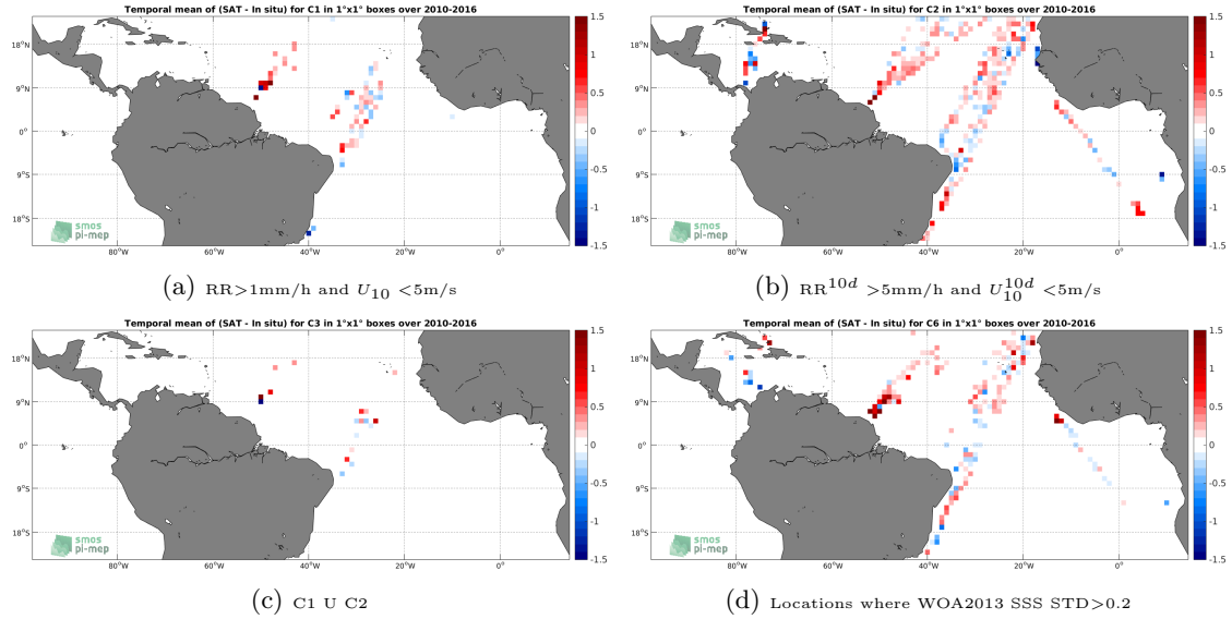
Figure 12: Temporal mean gridded over spatial boxes of size 1^\circ \times 1^\circ of \Delta SSS (SMOS-L3-ICDC-V3-MONTHLY-0.5DEG - TSG-LEGOS-DM) for 4 different subdatasets corresponding to:RR > 1 mm/h and U_{10} < 5 m/s (a), RR ^{10d} > 5 mm/h and U_{10}^{10d} < 5 m/s (b), C1 U C2 (c),Locations where WOA2013 SSS STD > 0.2 (d).
