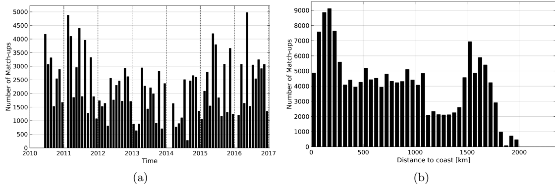
Figure 1: Number of match-ups between TSG-LEGOS-DM and SMOS-L3-ICDC-V3-MONTHLY-0.5DEG SSS as a function of time (a) and as function of the distance to coast (b) over the Tropical Atlantic Ocean Pi-MEP region and for the full satellite product period.
