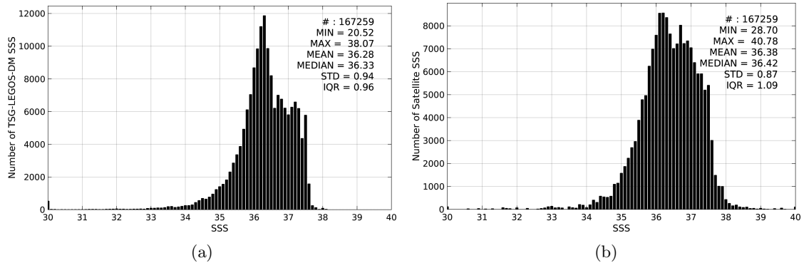
Figure 2: Histograms of SSS from TSG-LEGOS-DM (a) and SMOS-L3-ICDC-V3-MONTHLY-0.5DEG (b) considering all match-up pairs per bins of 0.1 over the Tropical Atlantic Ocean Pi-MEP region and for the full satellite product period.
