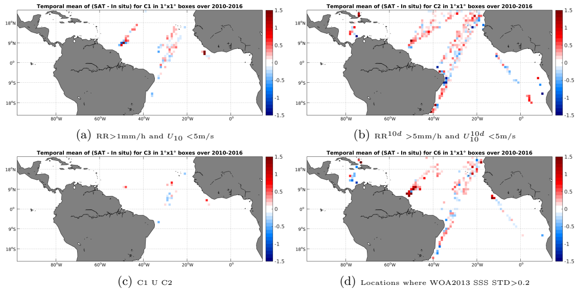
Figure 12: Temporal mean gridded over spatial boxes of size 1^\circ \times 1^\circ of \Delta SSS (SMOS-L3-ICDC-V3-MONTHLY-0.5DEG - TSG-LEGOS-DM) for 4 different subdatasets corresponding to: RR > 1\text{mm/h} and U_{10} < 5\text{m/s} (a), RR^{10d} > 5\text{mm/h} and U_{10}^{10d} < 5\text{m/s} (b), C1 U C2 (c), Locations where WOA2013 SSS STD > 0.2 (d).
