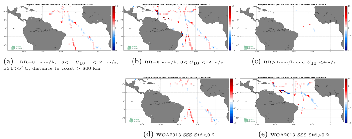
Figure 12: Temporal mean gridded over spatial boxes of size 1^\circ \times 1^\circ of \Delta\text{SSS} (SMOS SSS L3 v3 Monthly (ICDC) - TSG (GOSUD-Sailing-ship)) for 5 different subdatasets corresponding to:RR=0 mm/h, 3 < U_{10} < 12 m/s, SST>5°C, distance to coast > 800 km (a), RR=0 mm/h, 3 < U_{10} < 12 m/s (b), RR>1mm/h and U_{10} < 4 m/s (c), WOA2013 SSS Std<0.2 (d), WOA2013 SSS Std>0.2 (e).
