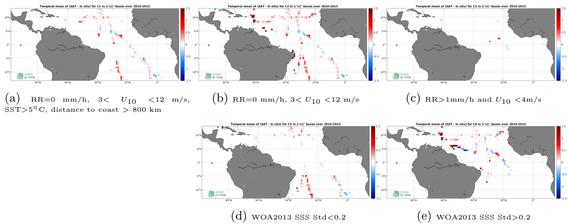
Figure 12: Temporal mean gridded over spatial boxes of size 1°x1° of \Delta SSS (SMOS SSS L3 v3 Monthly (ICDC) - TSG (GOSUD-Sailing-ship)) for 5 different subdatasets corresponding to:RR=0 mm/h, 3 < U_{10} < 12 m/s, SST>5°C, distance to coast > 800 km (a), RR=0 mm/h, 3 < U_{10} < 12 m/s (b), RR>1mm/h and U_{10} < 4 m/s (c), WOA2013 SSS Std<0.2 (d), WOA2013 SSS Std>0.2 (e).
