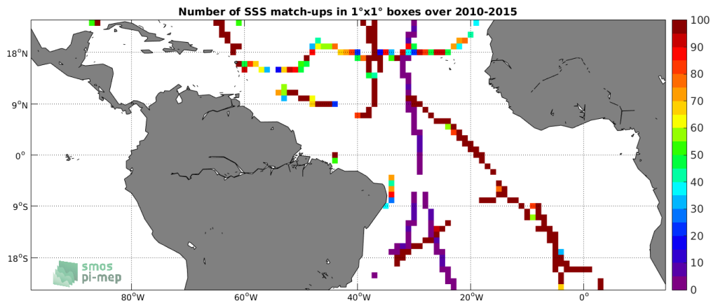
Figure 4: Number of SSS match-ups between TSG-GOSUD-Sailing-ship SSS and the SMOS-L3-ICDC-V3-MONTHLY-0.5DEG SSS product for the Tropical Atlantic Ocean Pi-MEP region over 1°x1° boxes and for the full satellite product period.
