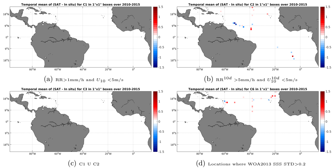
Figure 12: Temporal mean gridded over spatial boxes of size 1^\circ \times 1^\circ of \Delta SSS (SMOS-L3-ICDC-V3-MONTHLY-0.5DEG - TSG-GOSUD-Sailing-ship) for 4 different subdatasets corresponding to:RR > 1 mm/h and U_{10} < 5 m/s (a), RR^{10d} > 5 mm/h and U_{10}^{10d} < 5 m/s (b), C1 U C2 (c),Locations where WOA2013 SSS STD > 0.2 (d).
