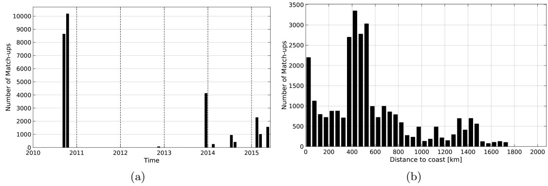
Figure 1: Number of match-ups between TSG-GOSUD-Sailing-ship and SMOS-L3-ICDC-V3-MONTHLY-0.5DEG SSS as a function of time (a) and as function of the distance to coast (b) over the Tropical Atlantic Ocean Pi-MEP region and for the full satellite product period.
