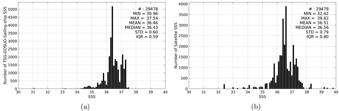
Figure 2: Histograms of SSS from TSG-GOSUD-Sailing-ship (a) and SMOS-L3-ICDC-V3-MONTHLY-0.5DEG (b) considering all match-up pairs per bins of 0.1 over the Tropical Atlantic Ocean Pi-MEP region and for the full satellite product period.
