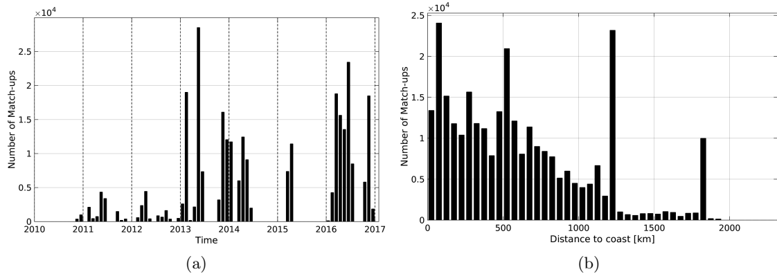
Figure 1: Number of match-ups between TSG-GOSUD-Research-vessel and SMOS-L3-ICDC-V3-MONTHLY-0.5DEG SSS as a function of time (a) and as function of the distance to coast (b) over the Tropical Atlantic Ocean Pi-MEP region and for the full satellite product period.
