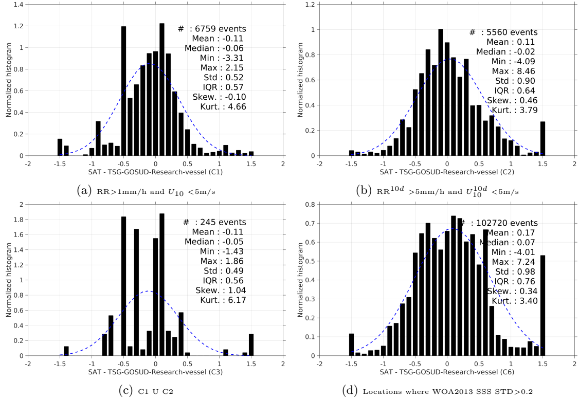
Figure 13: Normalized histogram of \Delta SSS (SMOS-L3-ICDC-V3-MONTHLY-0.5DEG - TSG-GOSUD-Research-vessel) for 6 different subdatasets corresponding to: RR > 1\text{mm/h} and U_{10} < 5\text{m/s} (a), RR^{10d} > 5\text{mm/h} and U_{10}^{10d} < 5\text{m/s} (b), C1 U C2 (c), Locations where WOA2013 SSS STD > 0.2 (d).
