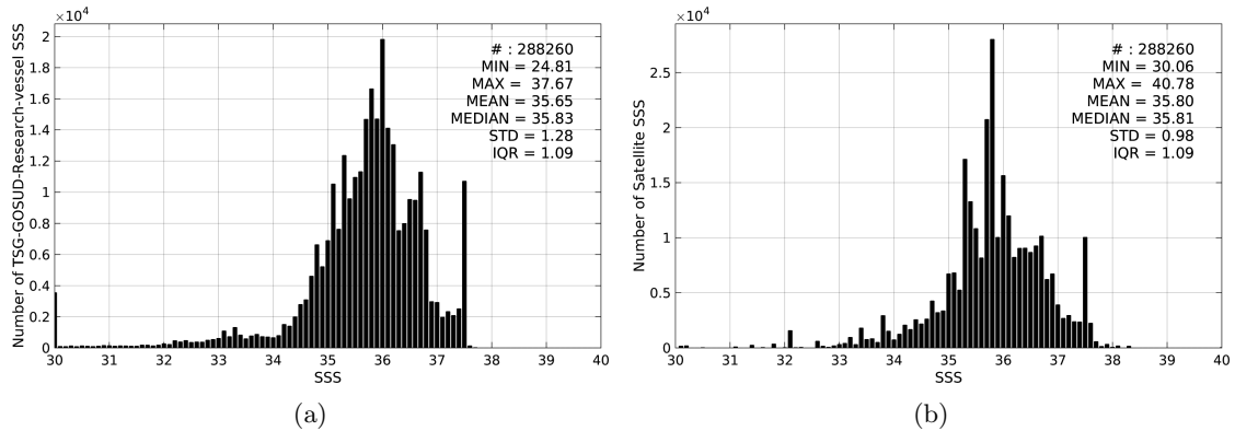
Figure 2: Histograms of SSS from TSG-GOSUD-Research-vessel (a) and SMOS-L3-ICDC-V3-MONTHLY-0.5DEG (b) considering all match-up pairs per bins of 0.1 over the Tropical Atlantic Ocean Pi-MEP region and for the full satellite product period.
