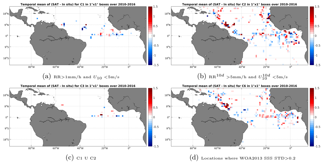
Figure 12: Temporal mean gridded over spatial boxes of size 1^\circ \times 1^\circ of \Delta SSS (SMOS-L3-ICDC-V3-MONTHLY-0.5DEG - TSG-GOSUD-Research-vessel) for 4 different subdatasets corresponding to:RR > 1 mm/h and U_{10} < 5 m/s (a), RR 10d > 5 mm/h and U_{10}^{10d} < 5 m/s (b), C1 U C2 (c),Locations where WOA2013 SSS STD > 0.2 (d).
