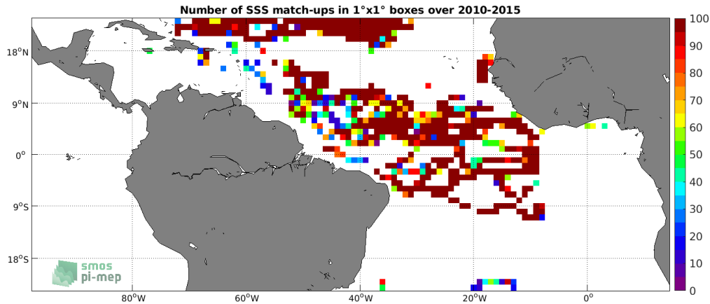
Figure 3: Number of SSS match-ups between Surface drifters SSS and the SMOS SSS L3 v3 Monthly (ICDC) SSS product for the Tropical Atlantic Ocean Pi-MEP region over 1^\circ \times 1^\circ boxes and for the full satellite product period.
