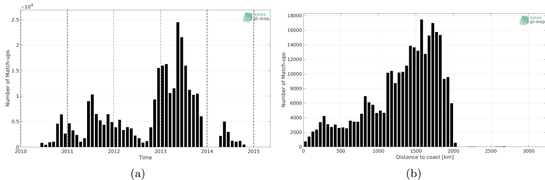
Figure 1: Number of match-ups between Surface drifters and SMOS SSS L3 v3 Monthly (ICDC) SSS as a function of time (a) and as function of the distance to coast (b) over the Tropical Atlantic Ocean Pi-MEP region and for the full satellite product period.
