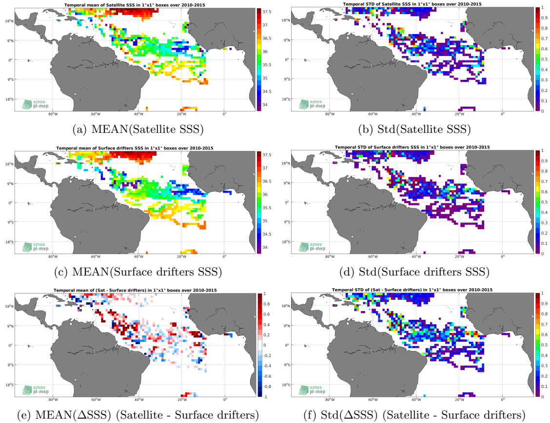
Figure 5: Temporal mean (left) and Std (right) of SSS from SMOS SSS L3 v3 Monthly (ICDC) (top), Surface drifters (middle), and of \Delta SSS (Satellite - Surface drifters). Only match-up pairs are used to generate these maps.
