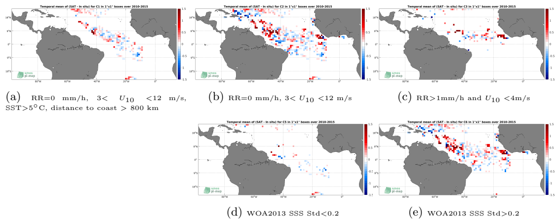
Figure 11: Temporal mean gridded over spatial boxes of size 1^\circ \times 1^\circ of \Delta\text{SSS} (SMOS SSS L3 v3 Monthly (ICDC) - Surface drifters) for 5 different subdatasets corresponding to:RR=0 mm/h, 3 < U_{10} < 12 m/s, SST > 5^\circ\text{C} , distance to coast > 800 km (a), RR=0 mm/h, 3 < U_{10} < 12 m/s (b), RR > 1 mm/h and U_{10} < 4 m/s (c), WOA2013 SSS Std < 0.2 (d), WOA2013 SSS Std > 0.2 (e).
