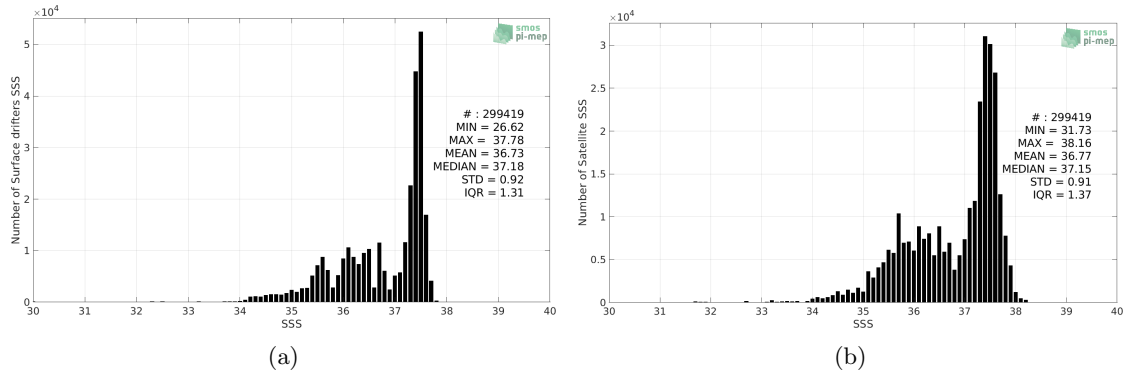
Figure 2: Histograms of SSS from Surface drifters (a) and SMOS SSS L3 v3 Monthly (ICDC) (b) considering all match-up pairs per bins of 0.1 over the Tropical Atlantic Ocean Pi-MEP region and for the full satellite product period.
