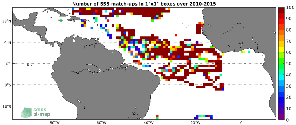
Figure 3: Number of SSS match-ups between Surface drifters SSS and the SMOS SSS L3 v3 Monthly (ICDC) SSS product for the Tropical Atlantic Ocean Pi-MEP region over 1°x1° boxes and for the full satellite product period.
