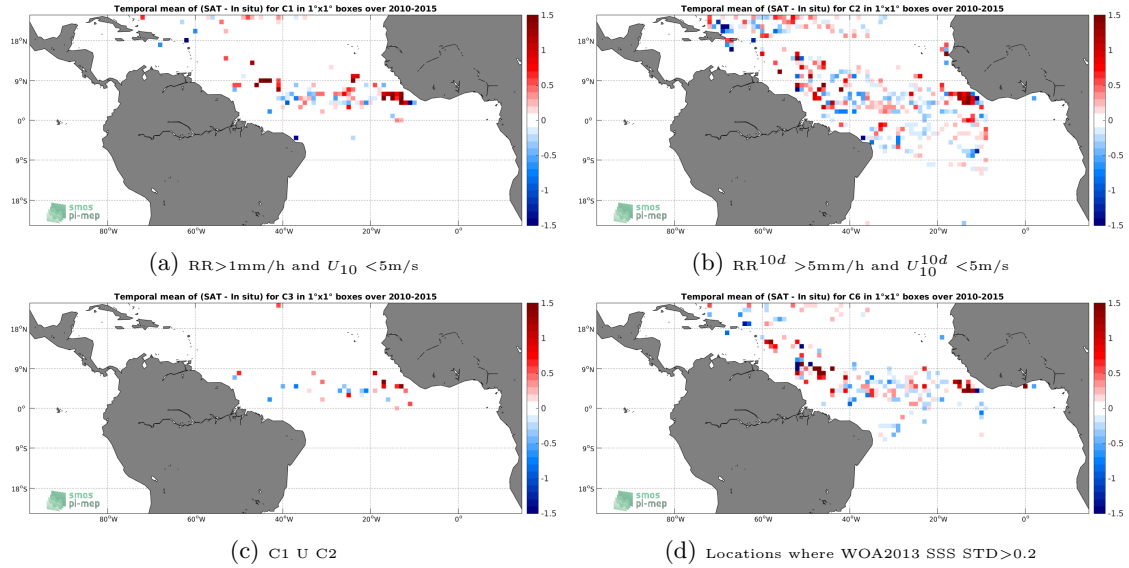
Figure 11: Temporal mean gridded over spatial boxes of size 1^\circ \times 1^\circ of \Delta SSS (SMOS-L3-ICDC-V3-MONTHLY-0.5DEG - Surface drifters) for 4 different subdatasets corresponding to:RR > 1 mm/h and U_{10} < 5 m/s (a), RR 10d > 5 mm/h and U_{10}^{10d} < 5 m/s (b), C1 U C2 (c),Locations where WOA2013 SSS STD > 0.2 (d).
