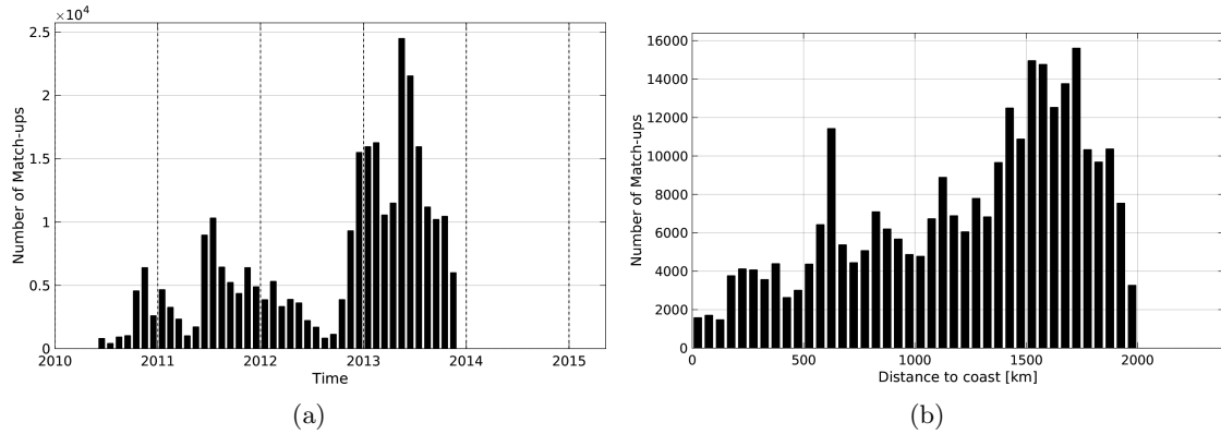
Figure 1: Number of match-ups between Surface drifters and SMOS-L3-ICDC-V3-MONTHLY-0.5DEG SSS as a function of time (a) and as function of the distance to coast (b) over the Tropical Atlantic Ocean Pi-MEP region and for the full satellite product period.
