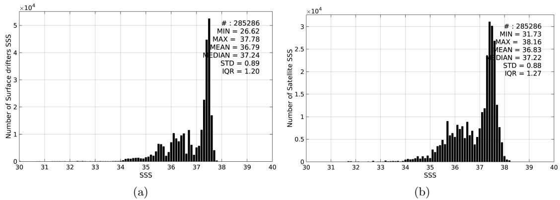
Figure 2: Histograms of SSS from Surface drifters (a) and SMOS-L3-ICDC-V3-MONTHLY-0.5DEG (b) considering all match-up pairs per bins of 0.1 over the Tropical Atlantic Ocean Pi-MEP region and for the full satellite product period.
