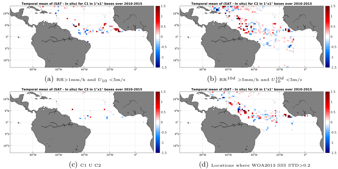
Figure 11: Temporal mean gridded over spatial boxes of size 1^\circ \times 1^\circ of \Delta SSS (SMOS-L3-ICDC-V3-MONTHLY-0.5DEG - Surface drifters) for 4 different subdatasets corresponding to:RR>1mm/h and U_{10} < 5\text{m/s} (a), RR^{10d} > 5\text{mm/h} and U_{10}^{10d} < 5\text{m/s} (b), C1 U C2 (c),Locations where WOA2013 SSS STD>0.2 (d).
