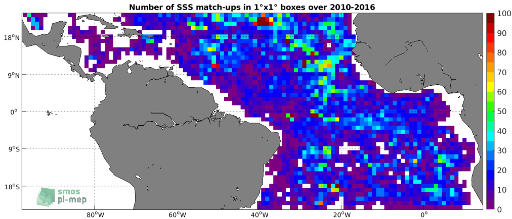
Figure 4: Number of SSS match-ups between Argo SSS and the SMOS SSS L3 v3 Monthly (ICDC) SSS product for the Tropical Atlantic Ocean Pi-MEP region over 1°x1° boxes and for the full satellite product period.
