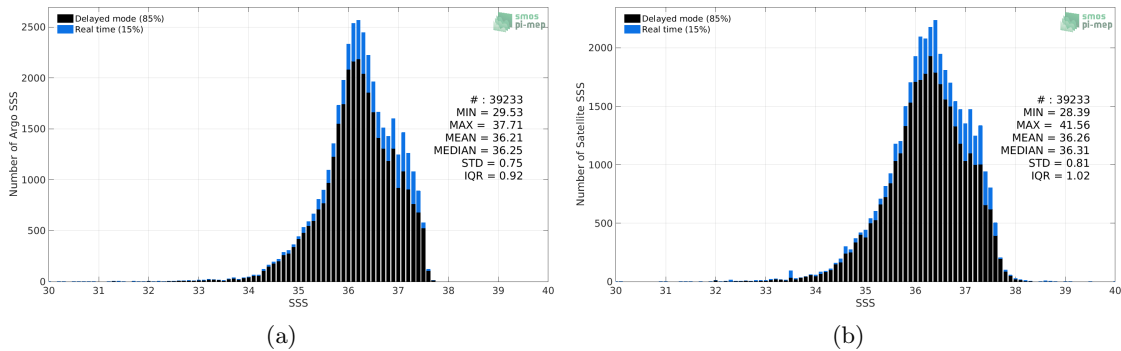
Figure 2: Histograms of SSS from Argo (a) and SMOS SSS L3 v3 Monthly (ICDC) (b) considering all match-up pairs per bins of 0.1 over the Tropical Atlantic Ocean Pi-MEP region and for the full satellite product period.
