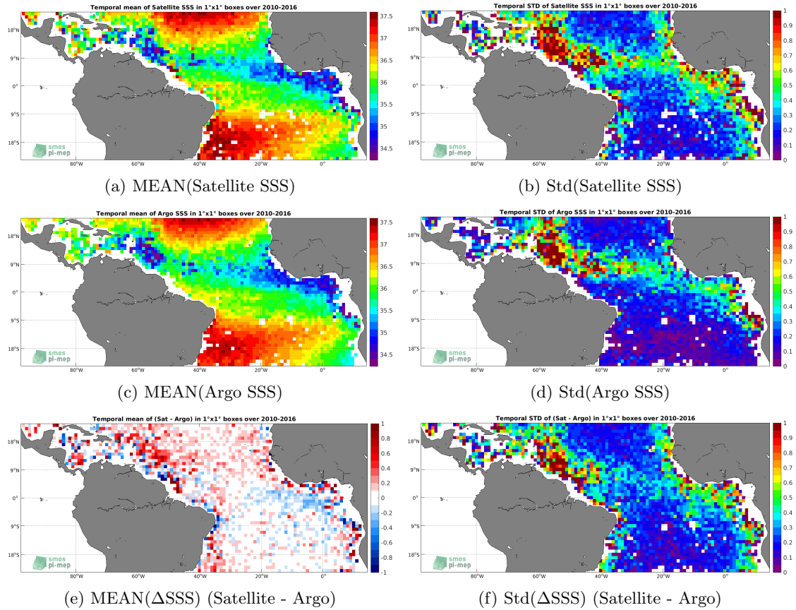
Figure 6: Temporal mean (left) and Std (right) of SSS from SMOS SSS L3 v3 Monthly (ICDC) (top), Argo (middle), and of \Delta SSS (Satellite - Argo). Only match-up pairs are used to generate these maps.
