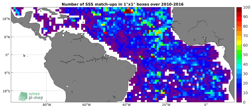
Figure 4: Number of SSS match-ups between Argo SSS and the SMOS SSS L3 v3 Monthly (ICDC) SSS product for the Tropical Atlantic Ocean Pi-MEP region over 1^\circ \times 1^\circ boxes and for the full satellite product period.
