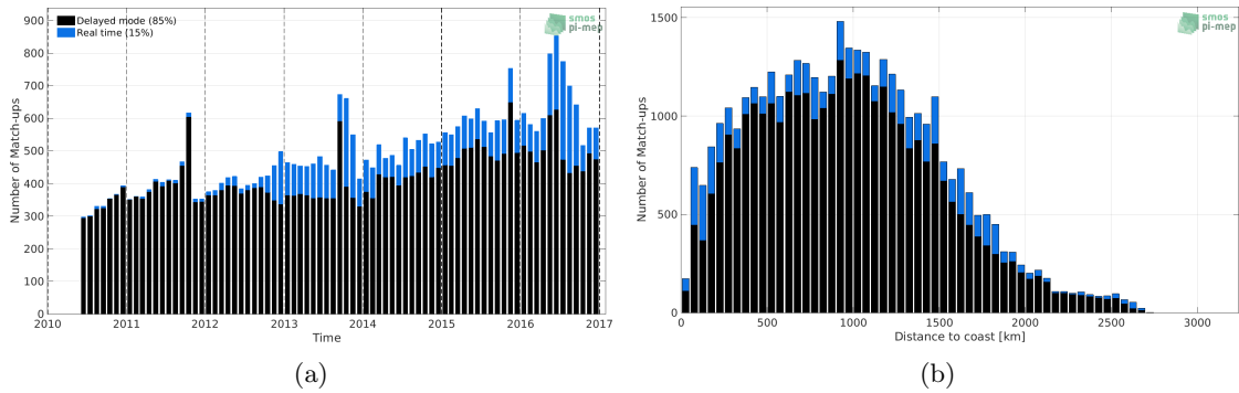
Figure 1: Number of match-ups between Argo and SMOS SSS L3 v3 Monthly (ICDC) SSS as a function of time (a) and as function of the distance to coast (b) over the Tropical Atlantic Ocean Pi-MEP region and for the full satellite product period.
