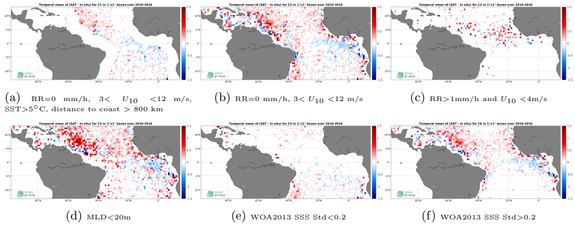
Figure 12: Temporal mean gridded over spatial boxes of size 1^\circ \times 1^\circ of \Delta SSS (SMOS SSS L3 v3 Monthly (ICDC) - Argo) for 6 different subdatasets corresponding to:RR=0 mm/h, 3 < U_{10} < 12 m/s, SST >5^\circ C, distance to coast > 800 km (a), RR=0 mm/h, 3 < U_{10} < 12 m/s (b), RR >1 mm/h and U_{10} < 4 m/s (c),MLD <20 m (d),WOA2013 SSS Std <0.2 (e),WOA2013 SSS Std >0.2 (f).
