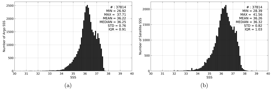
Figure 2: Histograms of SSS from Argo (a) and SMOS-L3-ICDC-V3-MONTHLY-0.5DEG (b) considering all match-up pairs per bins of 0.1 over the Tropical Atlantic Ocean Pi-MEP region and for the full satellite product period.
