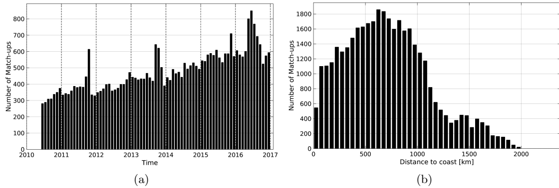
Figure 1: Number of match-ups between Argo and SMOS-L3-ICDC-V3-MONTHLY-0.5DEG SSS as a function of time (a) and as function of the distance to coast (b) over the Tropical Atlantic Ocean Pi-MEP region and for the full satellite product period.
