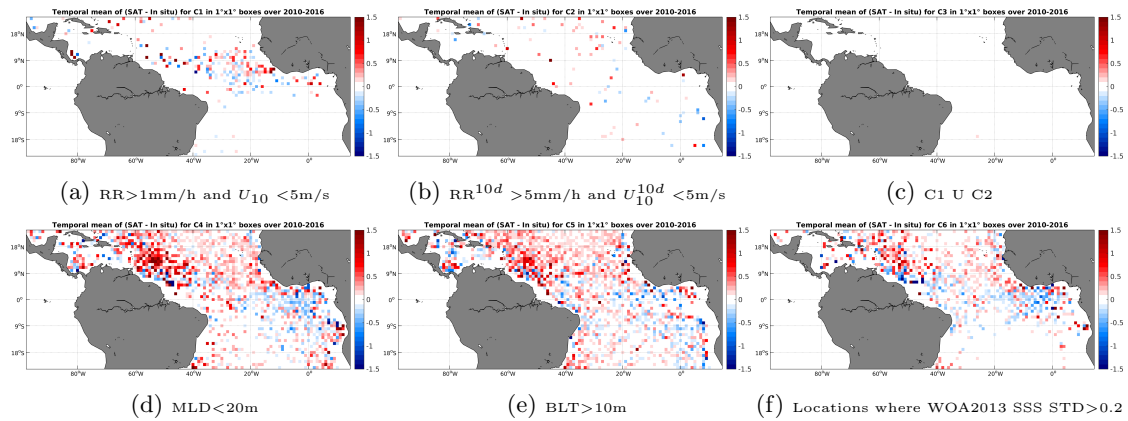
Figure 12: Temporal mean gridded over spatial boxes of size 1^\circ \times 1^\circ of \Delta SSS (SMOS-L3-ICDC-V3-MONTHLY-0.5DEG - Argo) for 6 different subdatasets corresponding to:RR >1 mm/h and U_{10} < 5 m/s (a), RR ^{10d} > 5 mm/h and U_{10}^{10d} < 5 m/s (b), C1 U C2 (c),MLD <20 m (d),BLT >10 m (e),Locations where WOA2013 SSS STD >0.2 (f).
