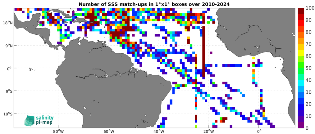
Figure 5: Number of SSS match-ups between TSG (SAMOS) SSS and the SMOS SSS L2Q v331 - With FLAG (CMEMS-CATDS-CPDC) SSS product for the Tropical Atlantic Ocean Pi-MEP region over 1^\circ \times 1^\circ boxes and for the full satellite product period.
