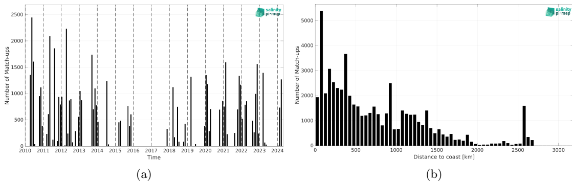
Figure 2: Number of match-ups between TSG (SAMOS) and SMOS SSS L2Q v331 - With FLAG (CMEMS-CATDS-CPDC) SSS as a function of time (a) and as function of the distance to coast (b) over the Tropical Atlantic Ocean Pi-MEP region and for the full satellite product period.
