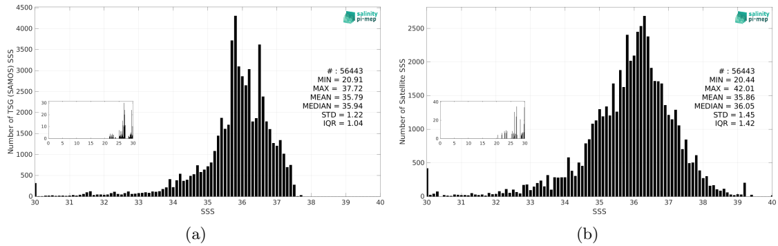
Figure 3: Histograms of SSS from TSG (SAMOS) (a) and SMOS SSS L2Q v331 - With FLAG (CMEMS-CATDS-CPDC) (b) considering all match-up pairs per bins of 0.1 over the Tropical Atlantic Ocean Pi-MEP region and for the full satellite product period.
