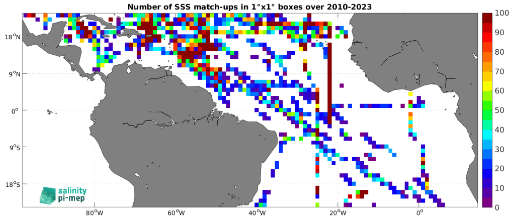
Figure 4: Number of SSS match-ups between TSG (SAMOS) SSS and the SMOS SSS L2Q v331 - With FLAG (CMEMS-CATDS-CPDC) SSS product for the Tropical Atlantic Ocean Pi-MEP region over 1^\circ \times 1^\circ boxes and for the full satellite product period.
