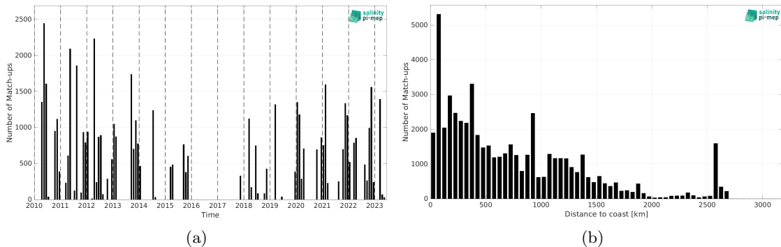
Figure 1: Number of match-ups between TSG (SAMOS) and SMOS SSS L2Q v331 - With FLAG (CMEMS-CATDS-CPDC) SSS as a function of time (a) and as function of the distance to coast (b) over the Tropical Atlantic Ocean Pi-MEP region and for the full satellite product period.
