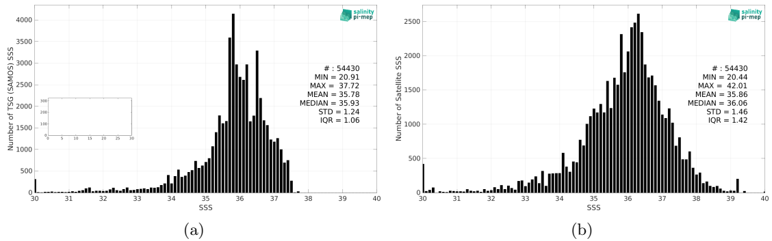
Figure 2: Histograms of SSS from TSG (SAMOS) (a) and SMOS SSS L2Q v331 - With FLAG (CMEMS-CATDS-CPDC) (b) considering all match-up pairs per bins of 0.1 over the Tropical Atlantic Ocean Pi-MEP region and for the full satellite product period.
