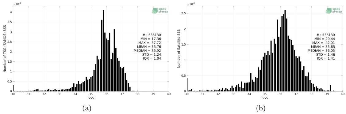
Figure 2: Histograms of SSS from TSG (SAMOS) (a) and SMOS SSS L2Q v331 - With FLAG (CMEMS-CATDS-CPDC) (b) considering all match-up pairs per bins of 0.1 over the Tropical Atlantic Ocean Pi-MEP region and for the full satellite product period.
