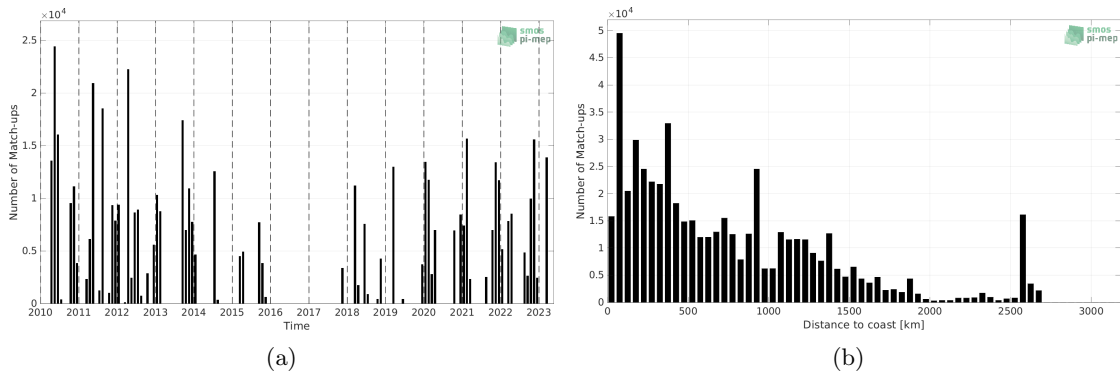
Figure 1: Number of match-ups between TSG (SAMOS) and SMOS SSS L2Q v331 - With FLAG (CMEMS-CATDS-CPDC) SSS as a function of time (a) and as function of the distance to coast (b) over the Tropical Atlantic Ocean Pi-MEP region and for the full satellite product period.
