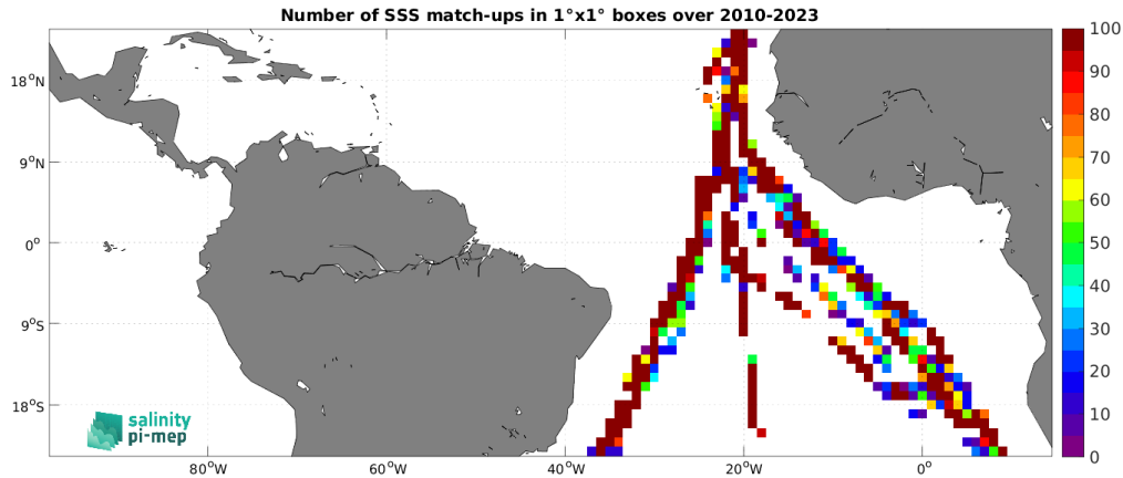
Figure 5: Number of SSS match-ups between TSG (Polarstern) SSS and the SMOS SSS L2Q v331 - With FLAG (CMEMS-CATDS-CPDC) SSS product for the Tropical Atlantic Ocean Pi-MEP region over 1^\circ \times 1^\circ boxes and for the full satellite product period.
