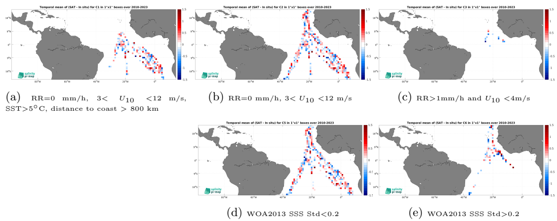
Figure 14: Temporal mean gridded over spatial boxes of size 1^\circ \times 1^\circ of \Delta SSS (SMOS SSS L2Q v331 - With FLAG (CMEMS-CATDS-CPDC) - TSG (Polarstern)) for 5 different subdatasets corresponding to:RR=0 mm/h, 3 < U_{10} < 12 m/s, SST >5^\circ C, distance to coast > 800 km (a), RR=0 mm/h, 3 < U_{10} < 12 m/s (b), RR >1 mm/h and U_{10} < 4 m/s (c), WOA2013 SSS Std <0.2 (d), WOA2013 SSS Std >0.2 (e).
