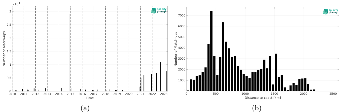
Figure 2: Number of match-ups between TSG (Polarstern) and SMOS SSS L2Q v331 - With FLAG (CMEMS-CATDS-CPDC) SSS as a function of time (a) and as function of the distance to coast (b) over the Tropical Atlantic Ocean Pi-MEP region and for the full satellite product period.
