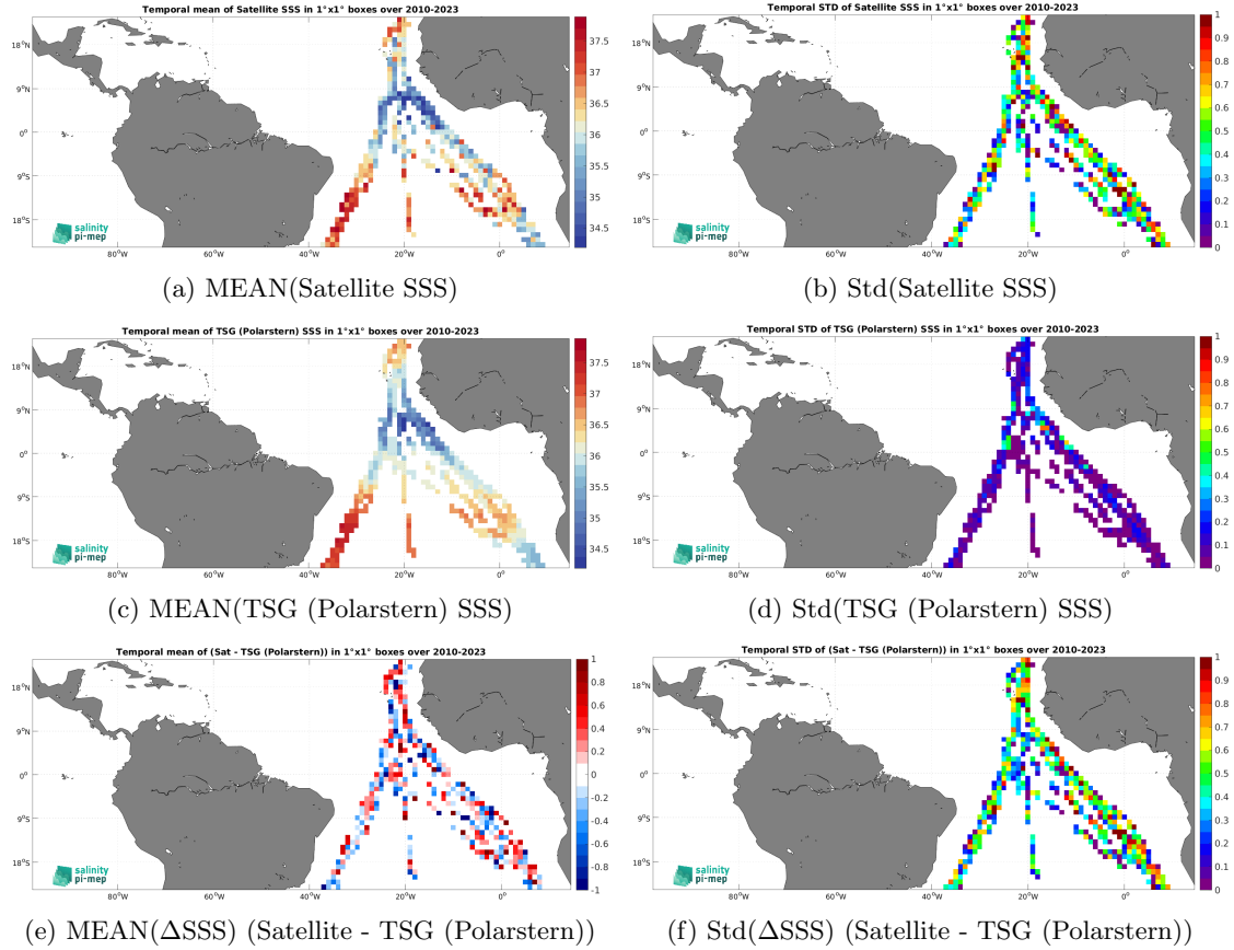
Figure 7: Temporal mean (left) and Std (right) of SSS from SMOS SSS L2Q v331 - With FLAG (CMEMS-CATDS-CPDC) (top), TSG (Polarstern) (middle), and of \Delta\text{SSS} (Satellite - TSG (Polarstern)). Only match-up pairs are used to generate these maps.
