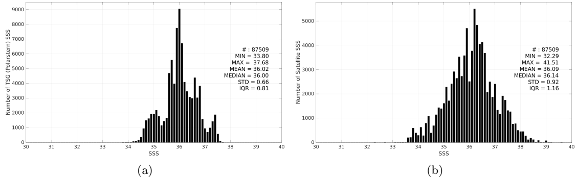
Figure 3: Histograms of SSS from TSG (Polarstern) (a) and SMOS SSS L2Q v331 - With FLAG (CMEMS-CATDS-CPDC) (b) considering all match-up pairs per bins of 0.1 over the Tropical Atlantic Ocean Pi-MEP region and for the full satellite product period.
