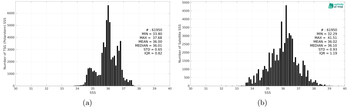
Figure 2: Histograms of SSS from TSG (Polarstern) (a) and SMOS SSS L2Q v331 - With FLAG (CMEMS-CATDS-CPDC) (b) considering all match-up pairs per bins of 0.1 over the Tropical Atlantic Ocean Pi-MEP region and for the full satellite product period.
