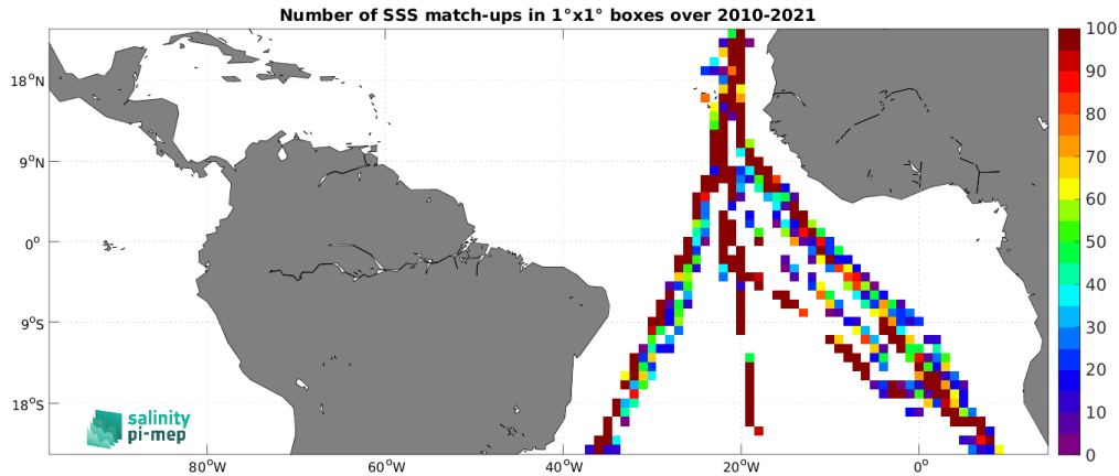
Figure 4: Number of SSS match-ups between TSG (Polarstern) SSS and the SMOS SSS L2Q v331 - With FLAG (CMEMS-CATDS-CPDC) SSS product for the Tropical Atlantic Ocean Pi-MEP region over 1^\circ \times 1^\circ boxes and for the full satellite product period.
