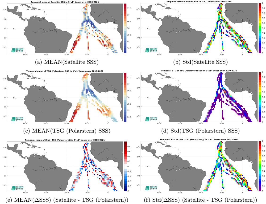
Figure 6: Temporal mean (left) and Std (right) of SSS from SMOS SSS L2Q v331 - With FLAG (CMEMS-CATDS-CPDC) (top), TSG (Polarstern) (middle), and of \Delta\text{SSS} (Satellite - TSG (Polarstern)). Only match-up pairs are used to generate these maps.
