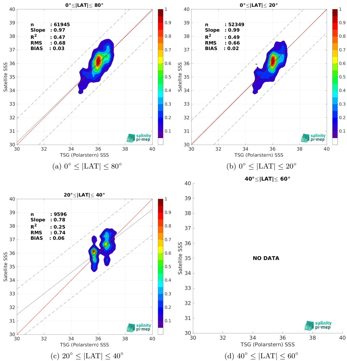
Figure 9: Contour maps of the concentration of SMOS SSS L2Q v331 - With FLAG (CMEMS-CATDS-CPDC) SSS (y-axis) versus TSG (Polarstern) SSS (x-axis) at match-up pairs for different latitude bands. For each plot, the red line shows x=y . The black thin and dashed lines indicate a linear fit through the data cloud and the \pm 95\% confidence levels, respectively. The number match-up pairs n , the slope and R^2 coefficient of the linear fit, the root mean square (RMS) and the mean bias between satellite and in situ data are indicated for each latitude band in each plots.
