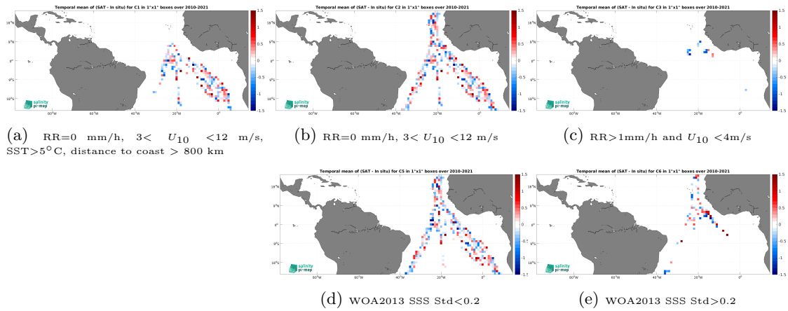
Figure 12: Temporal mean gridded over spatial boxes of size 1^{\circ}\times 1^{\circ} of \Delta\text{SSS} (SMOS SSS L2Q v331 - With FLAG (CMEMS-CATDS-CPDC) - TSG (Polarstern)) for 5 different subdatasets corresponding to:RR=0 mm/h, 3 < U_{10} < 12 m/s, SST > 5^{\circ}\text{C} , distance to coast > 800 km (a), RR=0 mm/h, 3 < U_{10} < 12 m/s (b), RR > 1 mm/h and U_{10} < 4 m/s (c), WOA2013 SSS Std < 0.2 (d), WOA2013 SSS Std > 0.2 (e).
