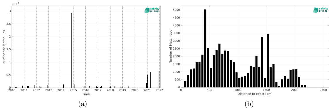
Figure 1: Number of match-ups between TSG (Polarstern) and SMOS SSS L2Q v331 - With FLAG (CMEMS-CATDS-CPDC) SSS as a function of time (a) and as function of the distance to coast (b) over the Tropical Atlantic Ocean Pi-MEP region and for the full satellite product period.
