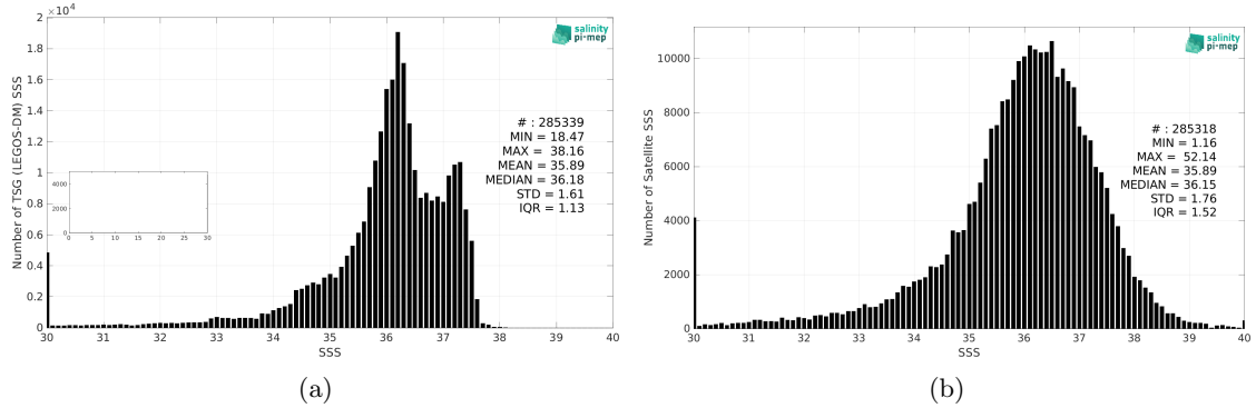
Figure 2: Histograms of SSS from TSG (LEGOS-DM) (a) and SMOS SSS L2Q v331 - With FLAG (CMEMS-CATDS-CPDC) (b) considering all match-up pairs per bins of 0.1 over the Tropical Atlantic Ocean Pi-MEP region and for the full satellite product period.
