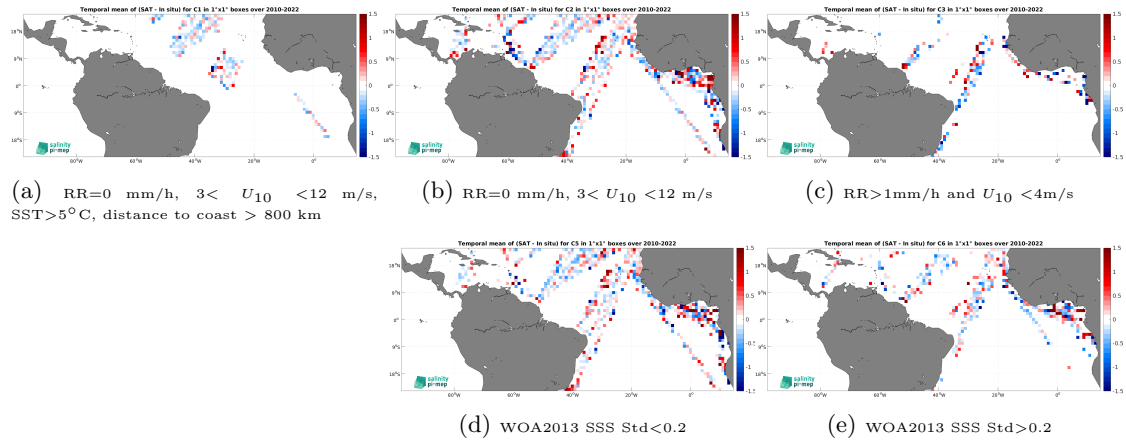
Figure 12: Temporal mean gridded over spatial boxes of size 1^\circ \times 1^\circ of \Delta\text{SSS} (SMOS SSS L2Q v331 - With FLAG (CMEMS-CATDS-CPDC) - TSG (LEGOS-DM)) for 5 different subdatasets corresponding to:RR=0 mm/h, 3 < U_{10} < 12 m/s, SST >5^\circ\text{C} , distance to coast > 800 km (a), RR=0 mm/h, 3 < U_{10} < 12 m/s (b), RR >1 mm/h and U_{10} < 4 m/s (c), WOA2013 SSS Std <0.2 (d), WOA2013 SSS Std >0.2 (e).
