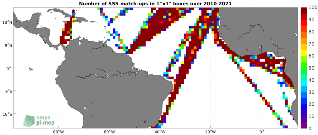
Figure 4: Number of SSS match-ups between TSG (LEGOS-DM) SSS and the SMOS SSS L2Q v331 - With FLAG (CMEMS-CATDS-CPDC) SSS product for the Tropical Atlantic Ocean Pi-MEP region over 1^\circ \times 1^\circ boxes and for the full satellite product period.
