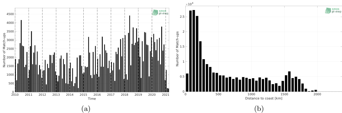
Figure 1: Number of match-ups between TSG (LEGOS-DM) and SMOS SSS L2Q v331 - With FLAG (CMEMS-CATDS-CPDC) SSS as a function of time (a) and as function of the distance to coast (b) over the Tropical Atlantic Ocean Pi-MEP region and for the full satellite product period.
