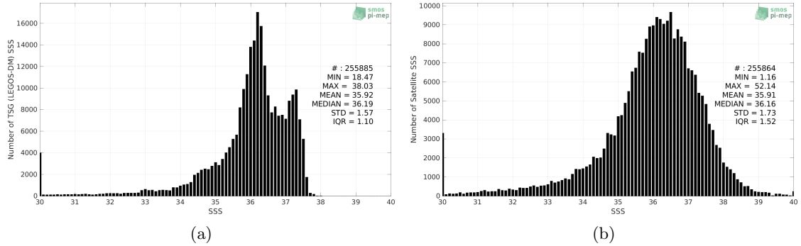
Figure 2: Histograms of SSS from TSG (LEGOS-DM) (a) and SMOS SSS L2Q v331 - With FLAG (CMEMS-CATDS-CPDC) (b) considering all match-up pairs per bins of 0.1 over the Tropical Atlantic Ocean Pi-MEP region and for the full satellite product period.
