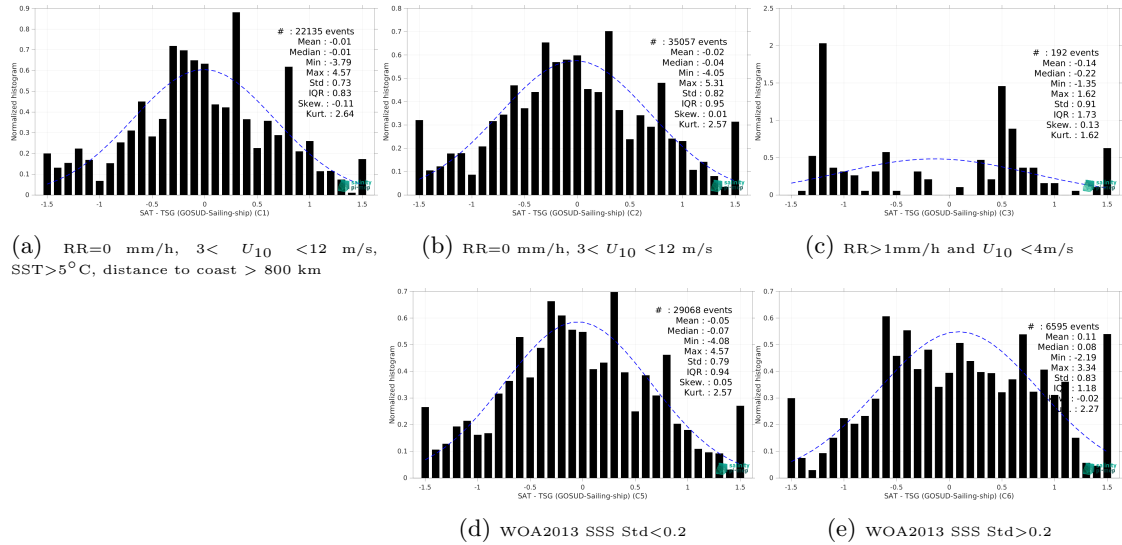
Figure 15: Normalized histogram of \Delta\text{SSS} (SMOS SSS L2Q v331 - With FLAG (CMEMS-CATDS-CPDC) - TSG (GOSUD-Sailing-ship)) for 5 different subdatasets corresponding to: RR=0 mm/h, 3 < U_{10} < 12 m/s, SST >5^{\circ}\text{C} , distance to coast > 800 km (a), RR=0 mm/h, 3 < U_{10} < 12 m/s (b), RR >1 mm/h and U_{10} < 4 m/s (c), WOA2013 SSS Std <0.2 (d), WOA2013 SSS Std >0.2 (e).
