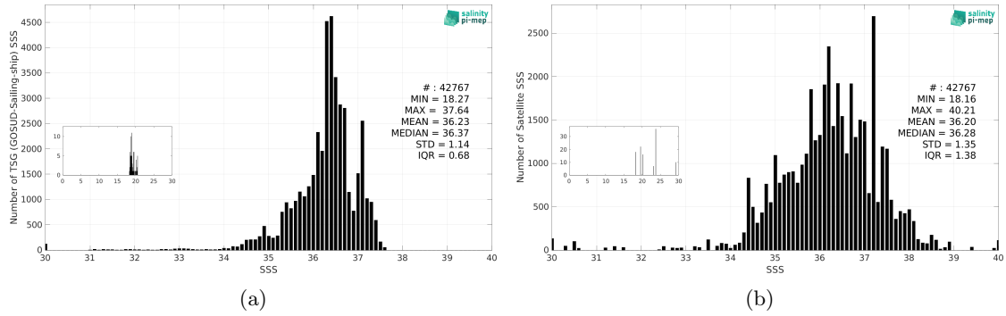
Figure 3: Histograms of SSS from TSG (GOSUD-Sailing-ship) (a) and SMOS SSS L2Q v331 - With FLAG (CMEMS-CATDS-CPDC) (b) considering all match-up pairs per bins of 0.1 over the Tropical Atlantic Ocean Pi-MEP region and for the full satellite product period.
