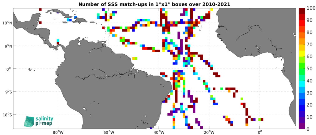
Figure 5: Number of SSS match-ups between TSG (GOSUD-Sailing-ship) SSS and the SMOS SSS L2Q v331 - With FLAG (CMEMS-CATDS-CPDC) SSS product for the Tropical Atlantic Ocean Pi-MEP region over 1^\circ \times 1^\circ boxes and for the full satellite product period.
