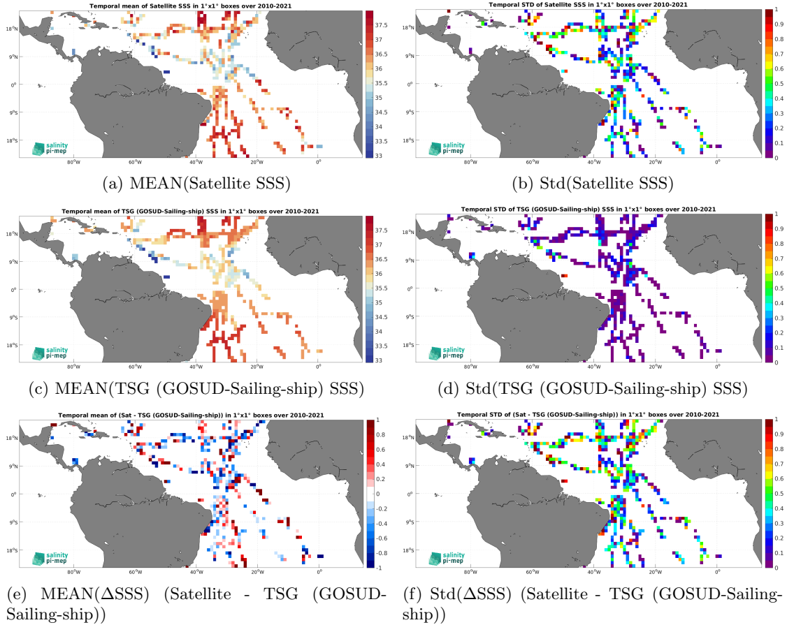
Figure 7: Temporal mean (left) and Std (right) of SSS from SMOS SSS L2Q v331 - With FLAG (CMEMS-CATDS-CPDC) (top), TSG (GOSUD-Sailing-ship) (middle), and of \Delta\text{SSS} (Satellite - TSG (GOSUD-Sailing-ship)). Only match-up pairs are used to generate these maps.
