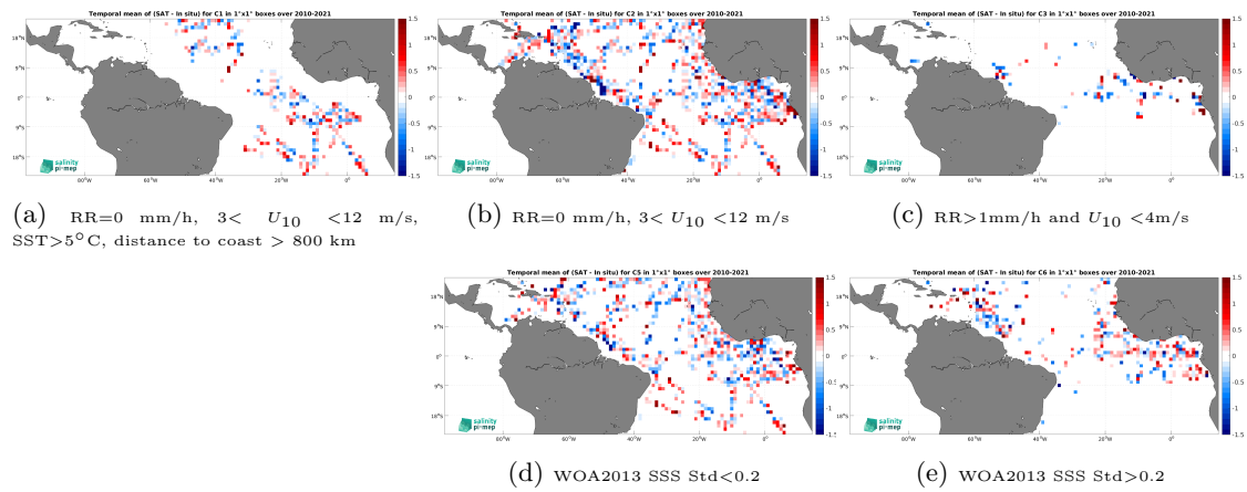
Figure 12: Temporal mean gridded over spatial boxes of size 1^\circ \times 1^\circ of \Delta\text{SSS} (SMOS SSS L2Q v331 - With FLAG (CMEMS-CATDS-CPDC) - TSG (GOSUD-Research-vessel)) for 5 different subdatasets corresponding to:RR=0 mm/h, 3 < U_{10} < 12 m/s, SST >5^\circ\text{C} , distance to coast > 800 km (a), RR=0 mm/h, 3 < U_{10} < 12 m/s (b), RR >1 mm/h and U_{10} < 4 m/s (c), WOA2013 SSS Std <0.2 (d), WOA2013 SSS Std >0.2 (e).
