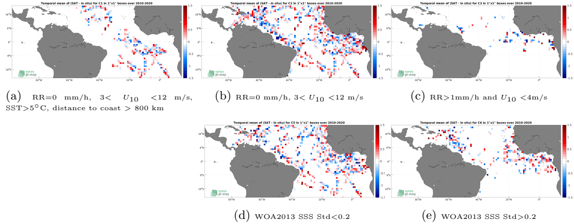
Figure 12: Temporal mean gridded over spatial boxes of size 1^{\circ}\times 1^{\circ} of \Delta SSS (SMOS SSS L2Q v331 - With FLAG (CMEMS-CATDS-CPDC) - TSG (GOSUD-Research-vessel)) for 5 different subdatasets corresponding to:RR=0 mm/h, 3 < U_{10} < 12 m/s, SST >5^{\circ}\text{C} , distance to coast > 800 km (a), RR=0 mm/h, 3 < U_{10} < 12 m/s (b), RR >1 mm/h and U_{10} < 4 m/s (c), WOA2013 SSS Std <0.2 (d), WOA2013 SSS Std >0.2 (e).
