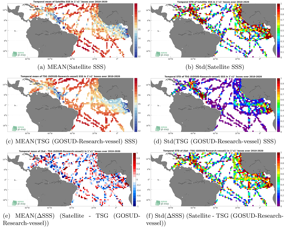
Figure 6: Temporal mean (left) and Std (right) of SSS from SMOS SSS L2Q v331 - With FLAG (CMEMS-CATDS-CPDC) (top), TSG (GOSUD-Research-vessel) (middle), and of \Delta\text{SSS} (Satellite - TSG (GOSUD-Research-vessel)). Only match-up pairs are used to generate these maps.
