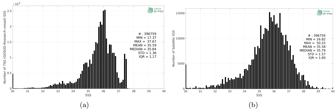
Figure 2: Histograms of SSS from TSG (GOSUD-Research-vessel) (a) and SMOS SSS L2Q v331 - With FLAG (CMEMS-CATDS-CPDC) (b) considering all match-up pairs per bins of 0.1 over the Tropical Atlantic Ocean Pi-MEP region and for the full satellite product period.
