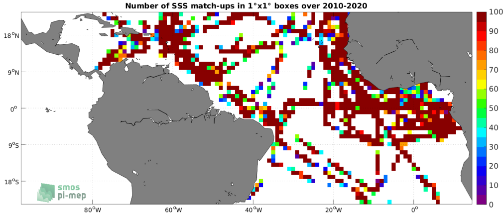
Figure 4: Number of SSS match-ups between TSG (GOSUD-Research-vessel) SSS and the SMOS SSS L2Q v331 - With FLAG (CMEMS-CATDS-CPDC) SSS product for the Tropical Atlantic Ocean Pi-MEP region over 1^\circ \times 1^\circ boxes and for the full satellite product period.
