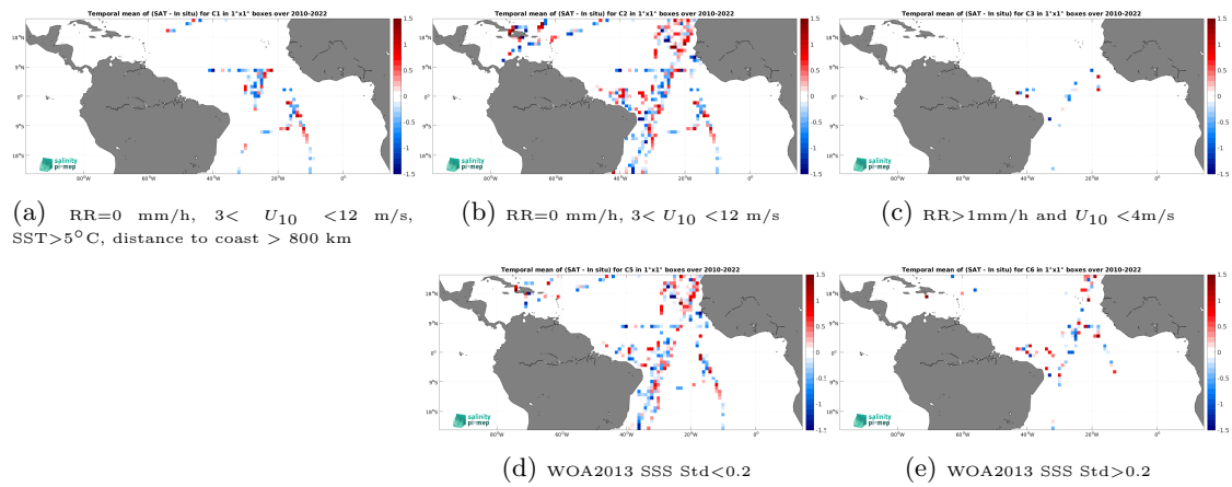
Figure 14: Temporal mean gridded over spatial boxes of size 1^\circ \times 1^\circ of \Delta\text{SSS} (SMOS SSS L2Q v331 - With FLAG (CMEMS-CATDS-CPDC) - TSG (CSIC-UTM)) for 5 different subdatasets corresponding to:RR=0 mm/h, 3 < U_{10} < 12 m/s, SST >5^\circ\text{C} , distance to coast > 800 km (a), RR=0 mm/h, 3 < U_{10} < 12 m/s (b), RR >1 mm/h and U_{10} < 4 m/s (c), WOA2013 SSS Std <0.2 (d), WOA2013 SSS Std >0.2 (e).
