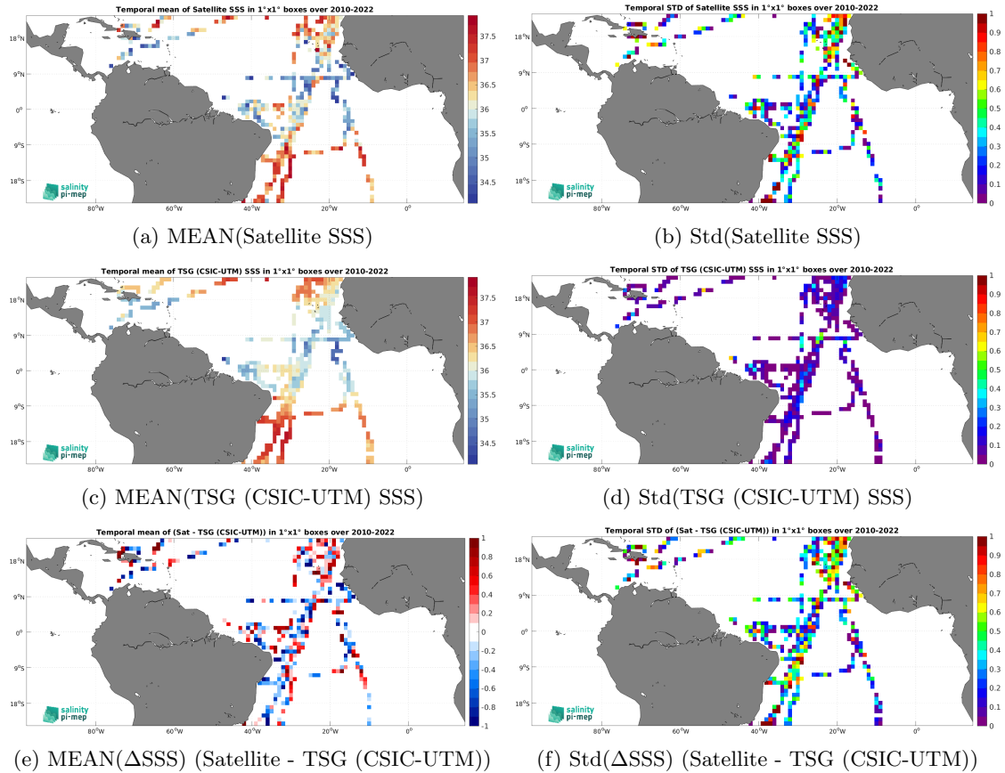
Figure 7: Temporal mean (left) and Std (right) of SSS from SMOS SSS L2Q v331 - With FLAG (CMEMS-CATDS-CPDC) (top), TSG (CSIC-UTM) (middle), and of \Delta\text{SSS} (Satellite - TSG (CSIC-UTM)). Only match-up pairs are used to generate these maps.
