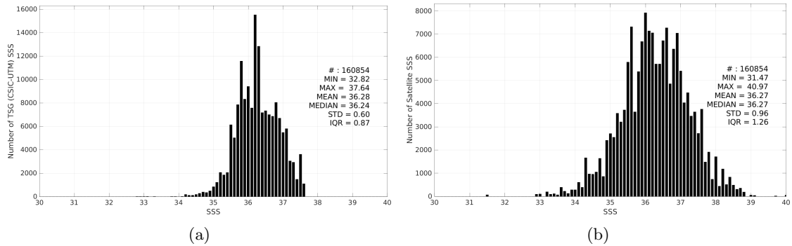
Figure 3: Histograms of SSS from TSG (CSIC-UTM) (a) and SMOS SSS L2Q v331 - With FLAG (CMEMS-CATDS-CPDC) (b) considering all match-up pairs per bins of 0.1 over the Tropical Atlantic Ocean Pi-MEP region and for the full satellite product period.
