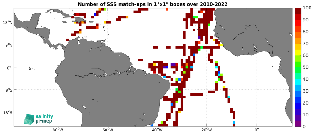
Figure 5: Number of SSS match-ups between TSG (CSIC-UTM) SSS and the SMOS SSS L2Q v331 - With FLAG (CMEMS-CATDS-CPDC) SSS product for the Tropical Atlantic Ocean Pi-MEP region over 1^\circ \times 1^\circ boxes and for the full satellite product period.
