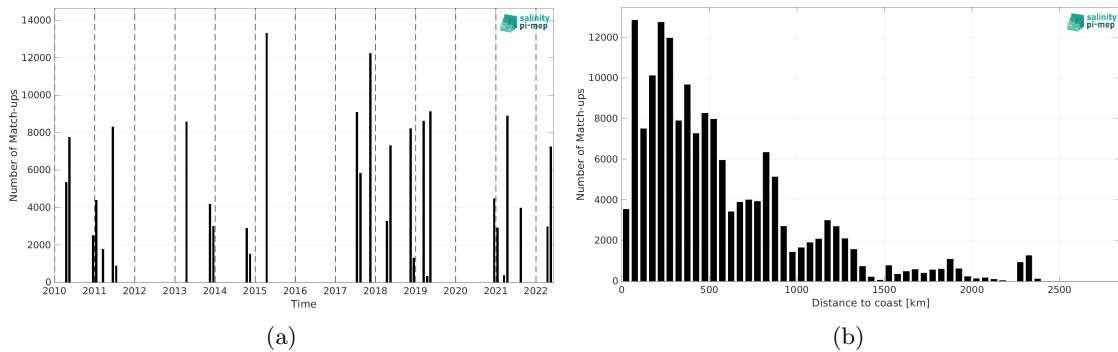
Figure 1: Number of match-ups between TSG (CSIC-UTM) and SMOS SSS L2Q v331 - With FLAG (CMEMS-CATDS-CPDC) SSS as a function of time (a) and as function of the distance to coast (b) over the Tropical Atlantic Ocean Pi-MEP region and for the full satellite product period.
