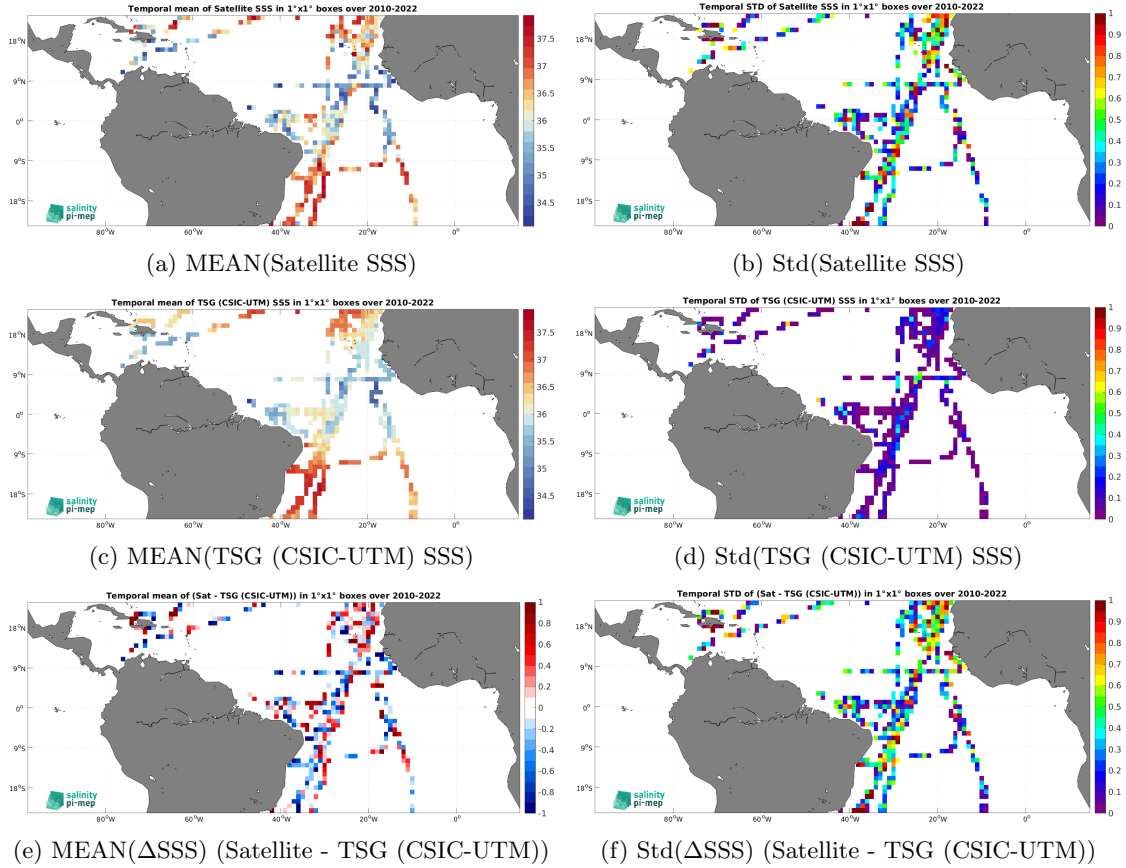
Figure 6: Temporal mean (left) and Std (right) of SSS from SMOS SSS L2Q v331 - With FLAG (CMEMS-CATDS-CPDC) (top), TSG (CSIC-UTM) (middle), and of \Delta\text{SSS} (Satellite - TSG (CSIC-UTM)). Only match-up pairs are used to generate these maps.
