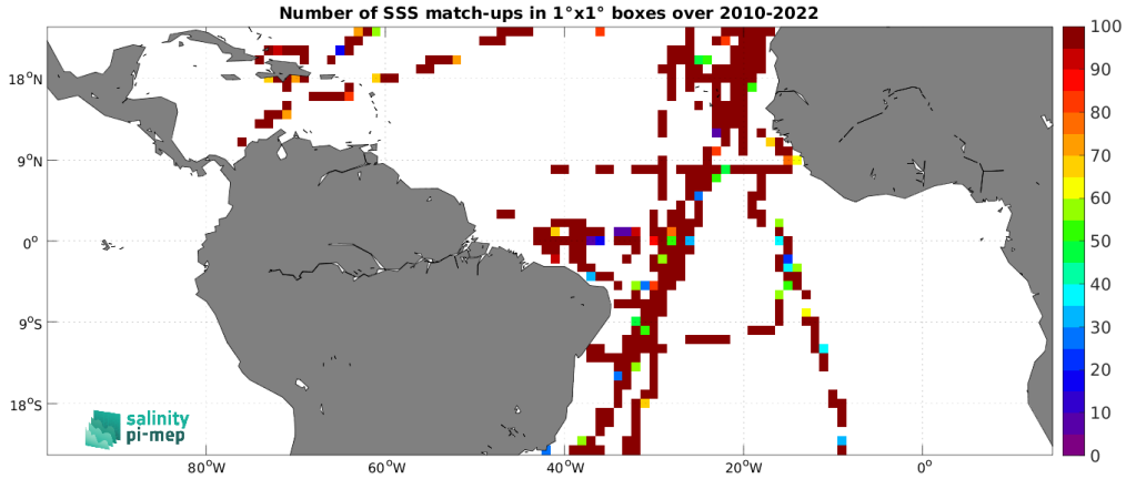
Figure 4: Number of SSS match-ups between TSG (CSIC-UTM) SSS and the SMOS SSS L2Q v331 - With FLAG (CMEMS-CATDS-CPDC) SSS product for the Tropical Atlantic Ocean Pi-MEP region over 1^\circ \times 1^\circ boxes and for the full satellite product period.
