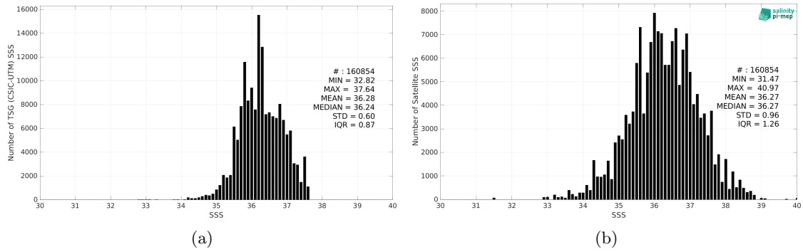
Figure 2: Histograms of SSS from TSG (CSIC-UTM) (a) and SMOS SSS L2Q v331 - With FLAG (CMEMS-CATDS-CPDC) (b) considering all match-up pairs per bins of 0.1 over the Tropical Atlantic Ocean Pi-MEP region and for the full satellite product period.
