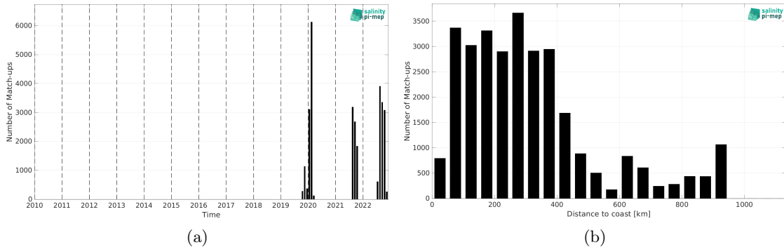
Figure 2: Number of match-ups between Saildrone and SMOS SSS L2Q v331 - With FLAG (CMEMS-CATDS-CPDC) SSS as a function of time (a) and as function of the distance to coast (b) over the Tropical Atlantic Ocean Pi-MEP region and for the full satellite product period.
