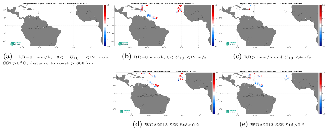
Figure 14: Temporal mean gridded over spatial boxes of size 1^\circ \times 1^\circ of \Delta SSS (SMOS SSS L2Q v331 - With FLAG (CMEMS-CATDS-CPDC) - Saildrone) for 5 different subdatasets corresponding to:RR=0 mm/h, 3 < U_{10} < 12 m/s, SST >5^\circ C, distance to coast > 800 km (a), RR=0 mm/h, 3 < U_{10} < 12 m/s (b), RR >1 mm/h and U_{10} < 4 m/s (c), WOA2013 SSS Std <0.2 (d), WOA2013 SSS Std >0.2 (e).
