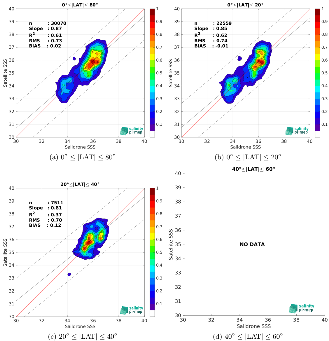
Figure 10: Contour maps of the concentration of SMOS SSS L2Q v331 - With FLAG (CMEMS-CATDS-CPDC) SSS (y-axis) versus Saildrone SSS (x-axis) at match-up pairs for different latitude bands. For each plot, the red line shows x=y . The black thin and dashed lines indicate a linear fit through the data cloud and the \pm 95\% confidence levels, respectively. The number match-up pairs n , the slope and R^2 coefficient of the linear fit, the root mean square (RMS) and the mean bias between satellite and in situ data are indicated for each latitude band in each plots.
