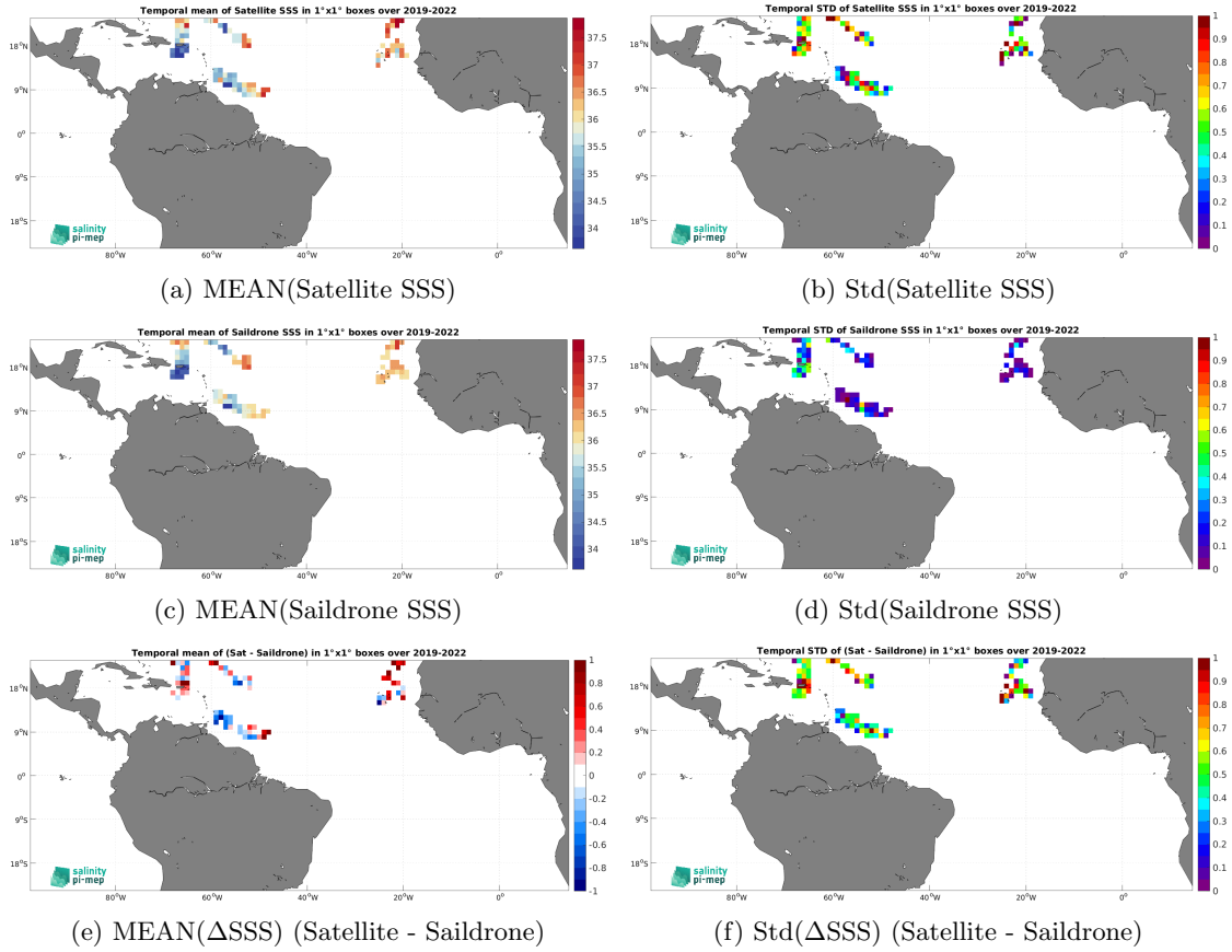
Figure 7: Temporal mean (left) and Std (right) of SSS from SMOS SSS L2Q v331 - With FLAG (CMEMS-CATDS-CPDC) (top), Sairdrone (middle), and of \Delta SSS (Satellite - Sairdrone). Only match-up pairs are used to generate these maps.
