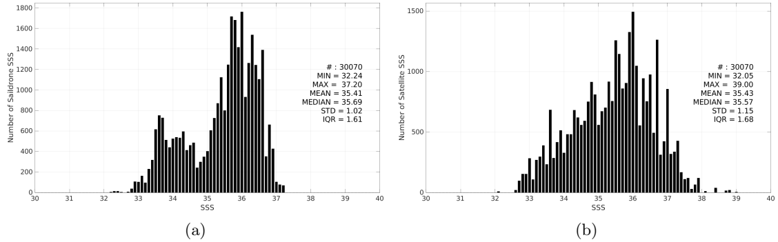
Figure 3: Histograms of SSS from Saildrone (a) and SMOS SSS L2Q v331 - With FLAG (CMEMS-CATDS-CPDC) (b) considering all match-up pairs per bins of 0.1 over the Tropical Atlantic Ocean Pi-MEP region and for the full satellite product period.
