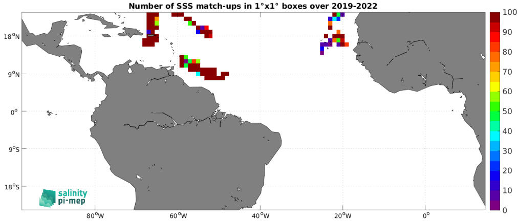
Figure 5: Number of SSS match-ups between Saildrone SSS and the SMOS SSS L2Q v331 - With FLAG (CMEMS-CATDS-CPDC) SSS product for the Tropical Atlantic Ocean Pi-MEP region over 1^\circ \times 1^\circ boxes and for the full satellite product period.
